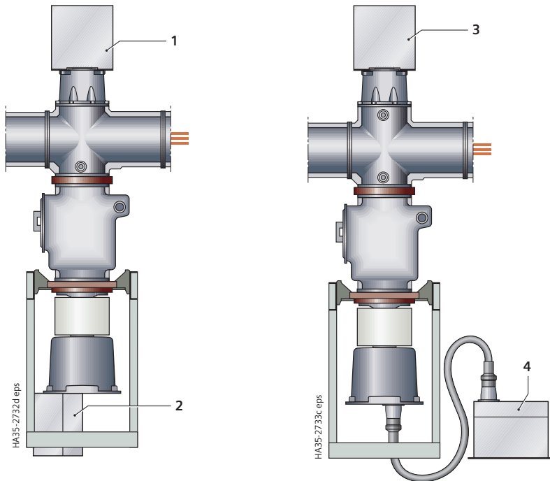
Voltage transformer installation (examples)
