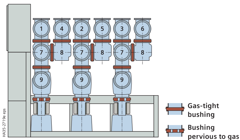
Double-busbar panel
