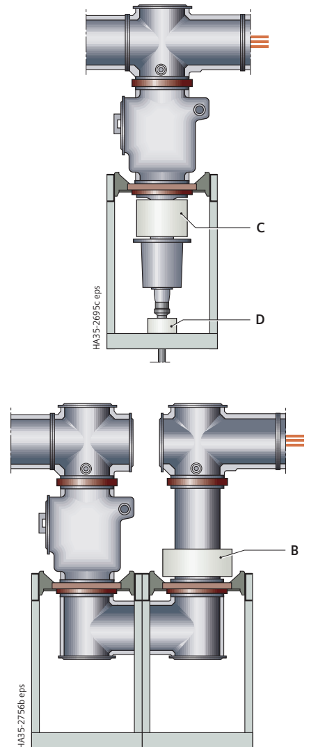
Current transformer installation (examples)
