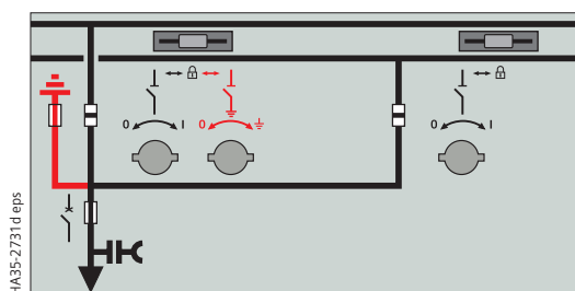
Feeder EARTHED
