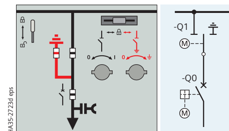
Feeder OPEN
