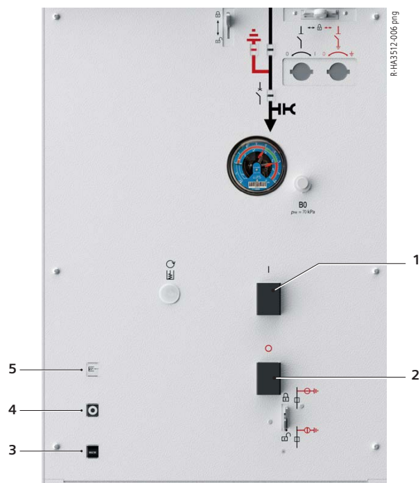
Circuit-breaker operating mechanism 3AH49 for single-busbar switchgear and double-busbar switchgear
