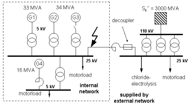
Figure 1: Generator stability
