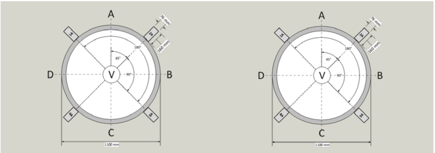
Sensor mounting options for 4-path measurements: reflect mode (left), direct X mode (right).
