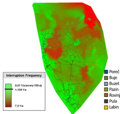
Figure 2: Calculated SAIFI values for each region in Elektroistra Pula.
