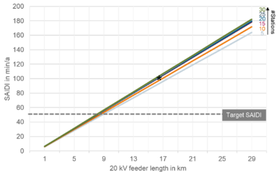
Figure 3: SAIDI depending on feeder length and number of secondary substations of a feeder.
