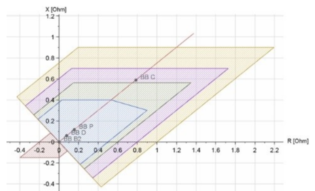
Figure 3: Impedance diagram including the line impedance
