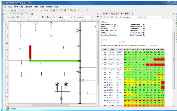
Figure 4: Concept verification with PSA
