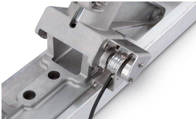
Sicat DMS-E: Rotary encoder unit on Sicat 8WL6144 disconnector
