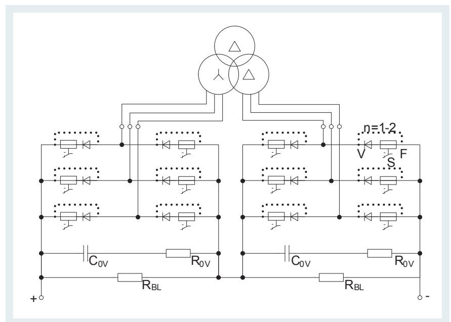
Series connection 6-pulse and 12-pulse version, DC 3000 V
