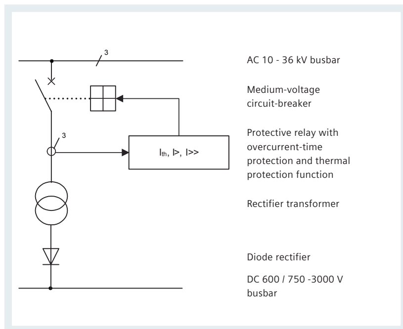
Schematic diagram: Protection against overload
