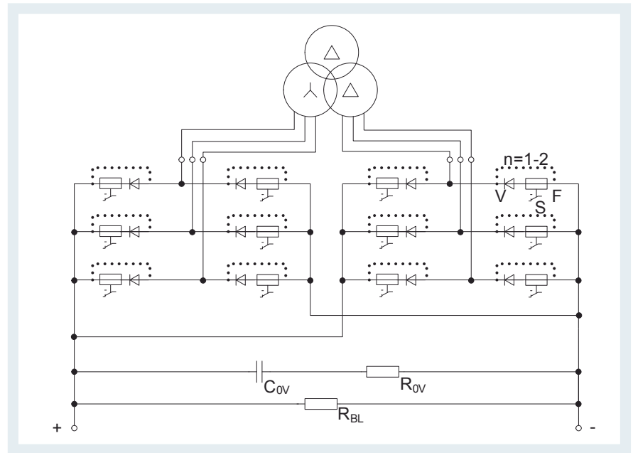
Parallel connection 6-pulse and 12-pulse version, DC 600 / 750 V and DC 1,500 V
