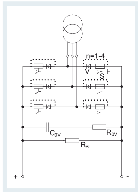
6-pulse version, DC 600 / 750 V and DC 1,500 V
