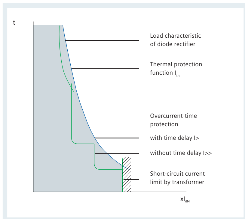
Schematic diagram: Protection against external short-circuit
