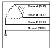
Figure 4 Delta & HRG Wye 3 Hots, 1 Grnd
