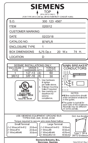
Example of Label provided on each enclosure with UL/cULus marking
