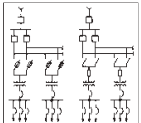
Figure 4. Primary Selective Systems
