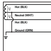
Figure 1 Split 2 Hots, 1 Neu, 1 Grnd
