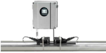
Sitrans FS230 clamp-on ultrasonic gas flow meter with non-intrusive sensors.
