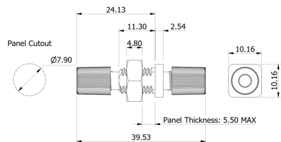
Figure 11: Optic Fibre Coupler dimensions
