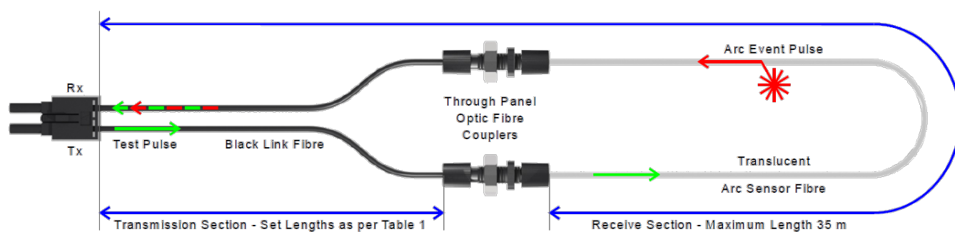
Figure 8: RA40 component function and installation limitations
