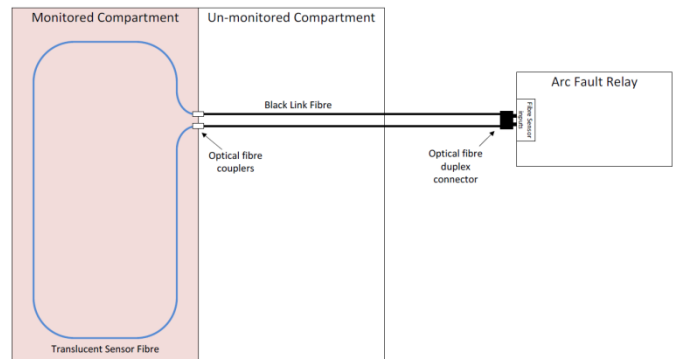
Figure 10: Diagram illustrating how neighboring compartments can be selectively monitored by passing the black clad link fibre through the compartment not to be monitored
