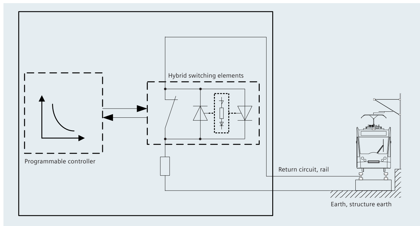
Block diagram Sitras SCD
