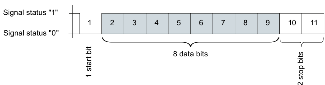
Figure 6-1 11-bit character frame
