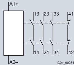
3RO 3SK1213 output expansion
