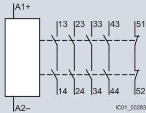
4RO 3SK1211 output expansion
