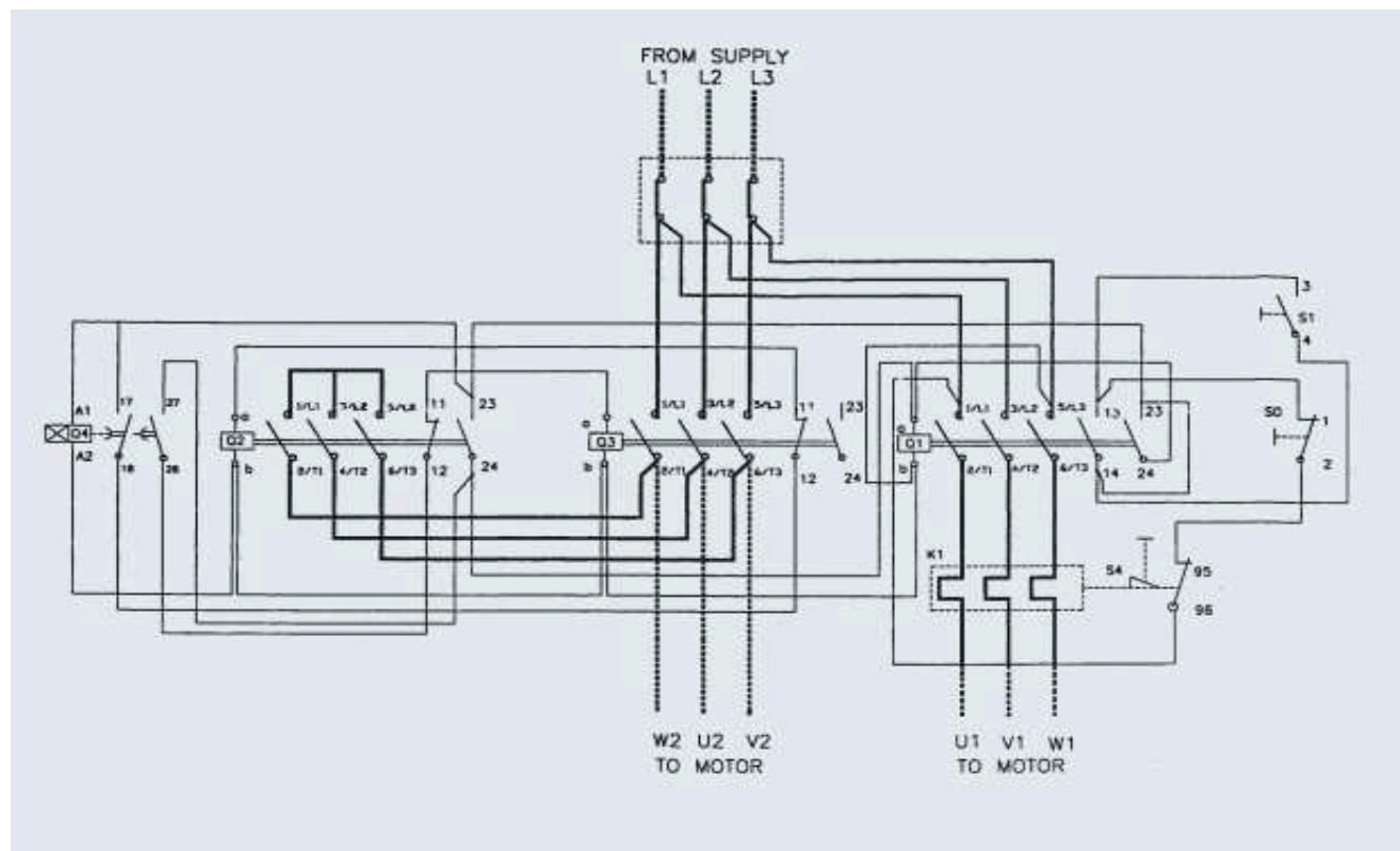
Figure 7: wiring Diagram
