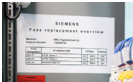
Figure 13-19 Example of marking for fuse holders
