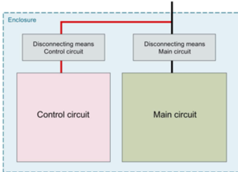
Figure 7-2 Control circuit tapped upstream of the main disconnecting means
