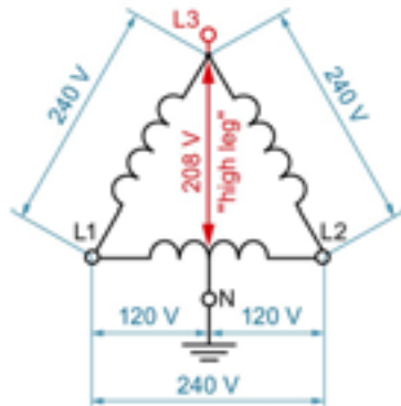
Figure 5-6 Midpoint grounded delta 240 V
