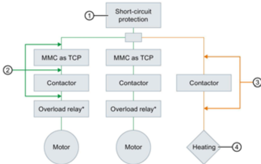
Figure 6-13 Group installation with tap conductor protection method 2
