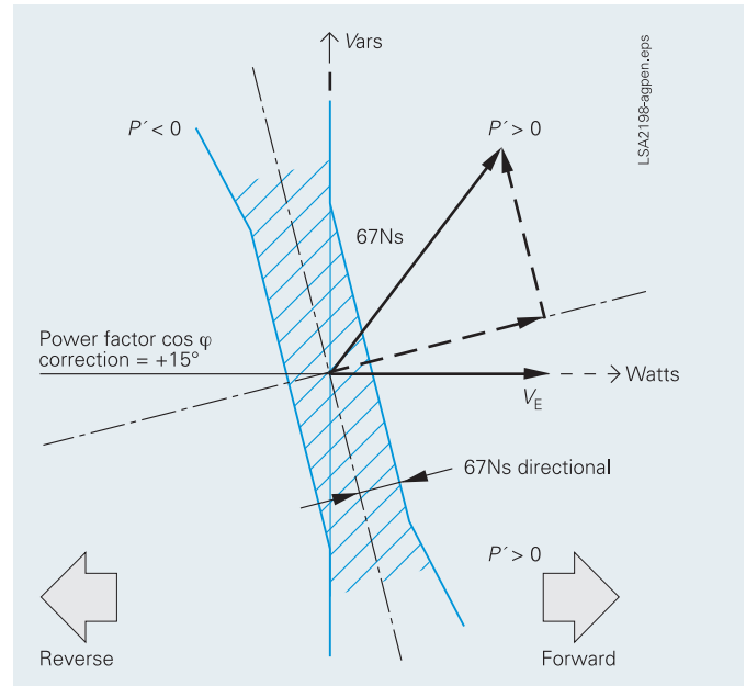
Fig. 5/39 Directional determination using cosine measurements
