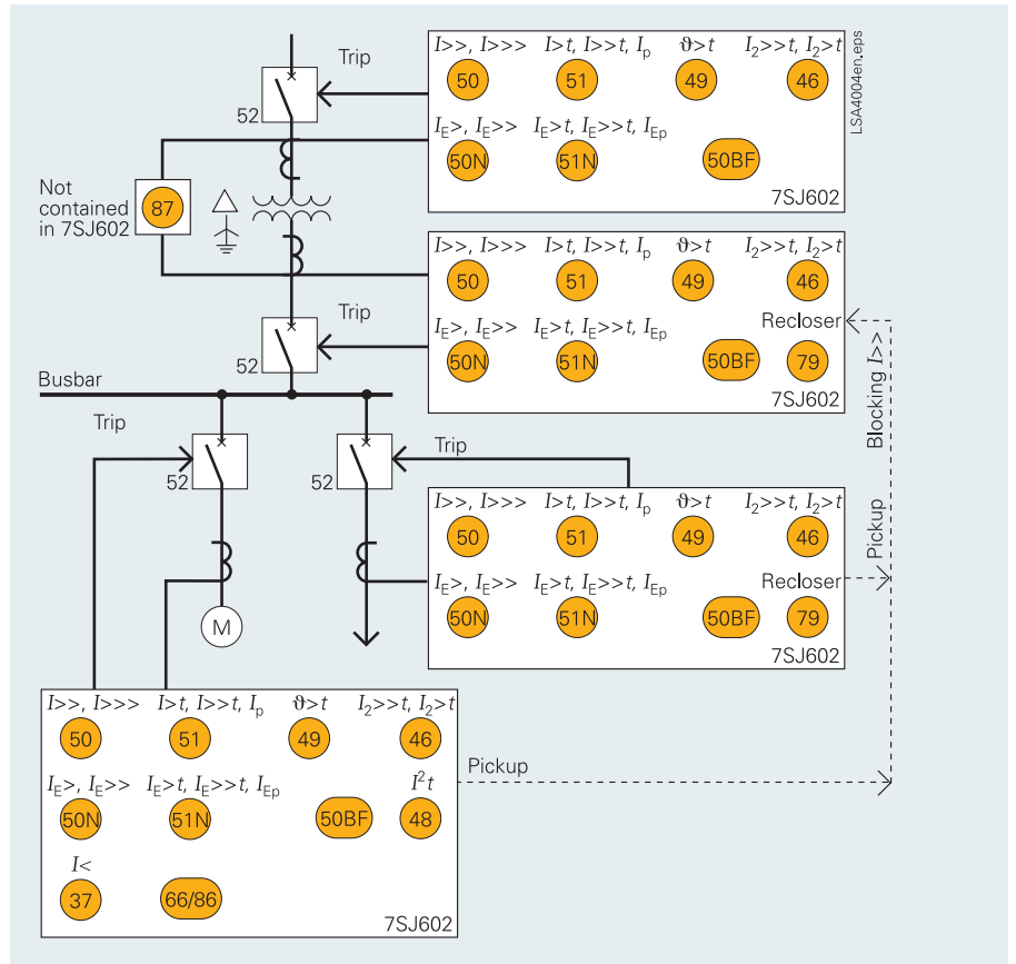
Fig. 5/41 Reserve interlocking
