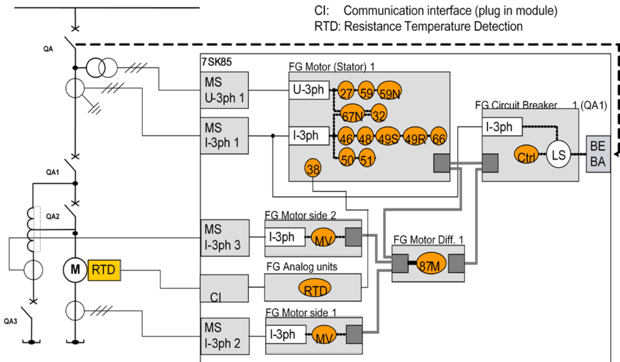
Fig. 4: 7SK85 Motor Differential Protection with additional CT and additional Function Group Motor Side
