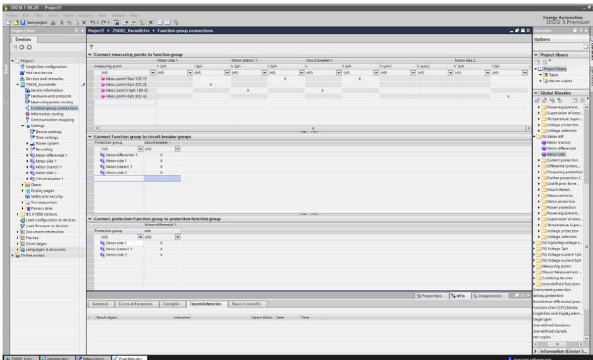
Fig. 6: 7SK85 – Function Group Connection in DIGSI 5
