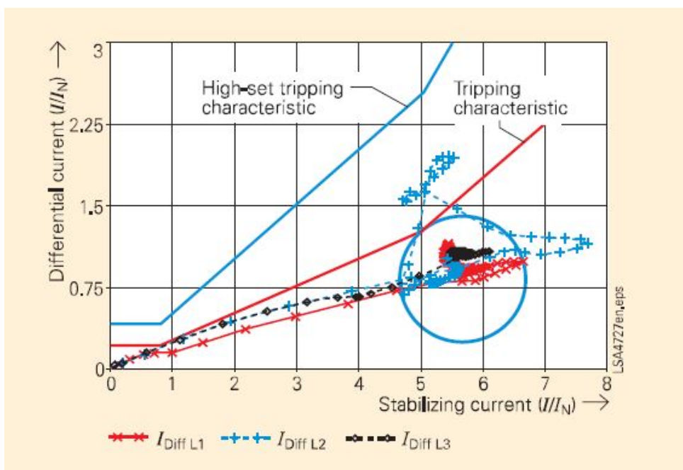
Fig.2: Differential currents during motor starting (approx. 5sec) [2]
