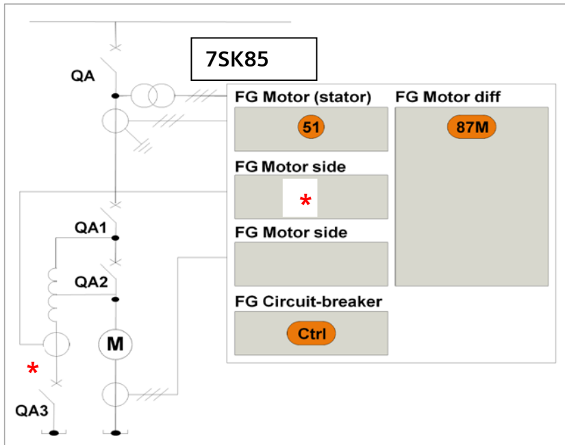
Fig.3: 7SK85 Motor Protection with Korndorfer Starter; (*additional CT, additional Function Group)
