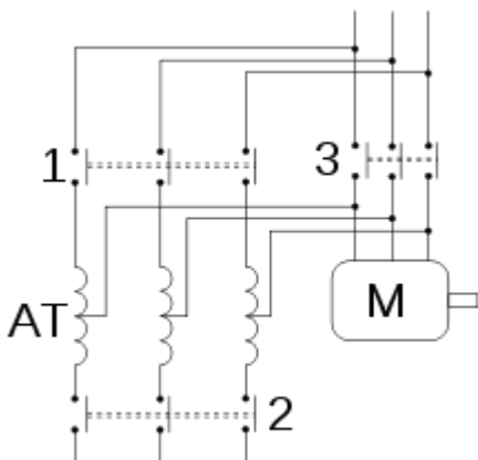
Fig. 1: Korndorfer starter with motor (M), autotransformer (AT) and three switches (1, 2, 3)
