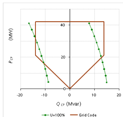
Figure 1: Example of reactive power capability curves
