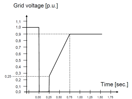
Figure 2: Example of a fault ride-through requirement curve
