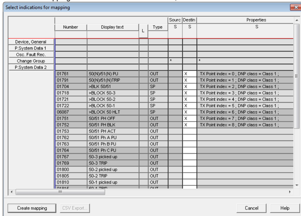
Figure 3-2 Creation of a Mapping
