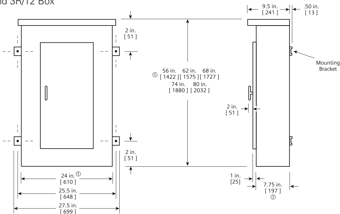
Type 3R and 3R/12 Box
