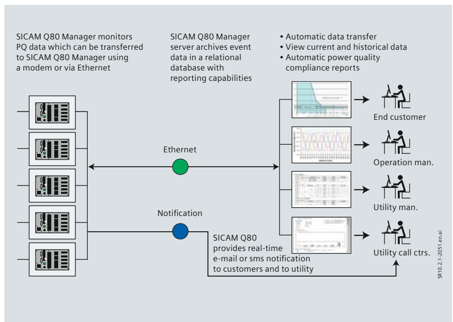
Fig. 4/14 SICAM Q80 – system overview
