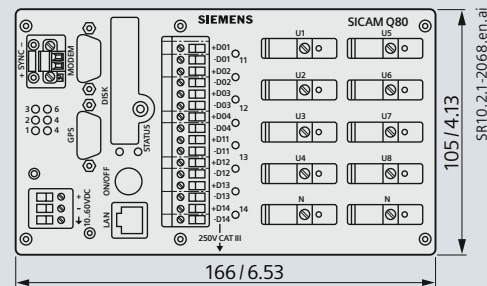
Fig. 4/32 7KG8080 – eight-voltage connection: front view
