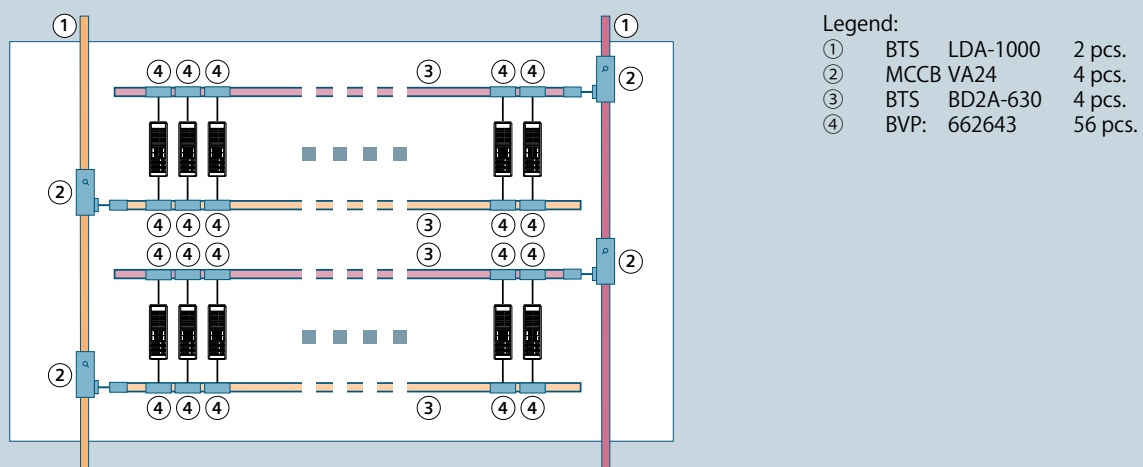
Fig. 4: Version 2: Server room (approx. 600 kVA) with 3-phase rack supply (maximum rack power demand of 22 kVA)
