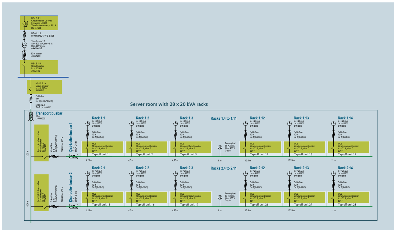
Fig. 6: Version 2: Server room (approx. 560 kVA) with 3-phase rack supply (maximum rack power demand of 20 kVA)
