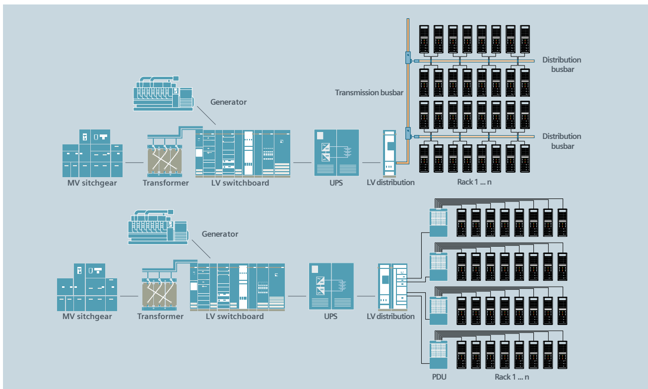
Fig. 1: Comparison of power distribution solutions with cables or busbar trunking systems (BTS) in the data center
