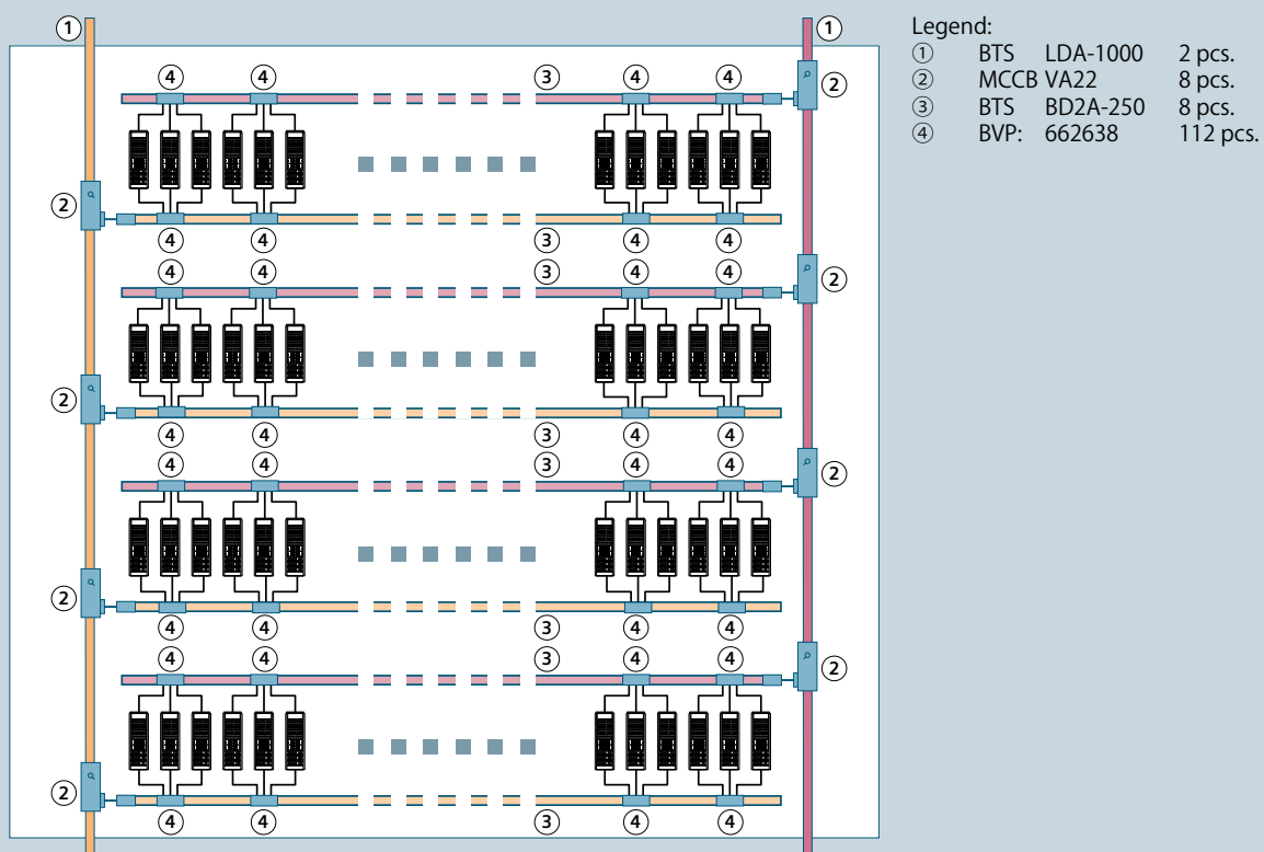
Fig. 3: Version 1: Server room (approx. 600 kVA) with 1-phase rack supply (maximum rack power demand of 3.6 kVA)
