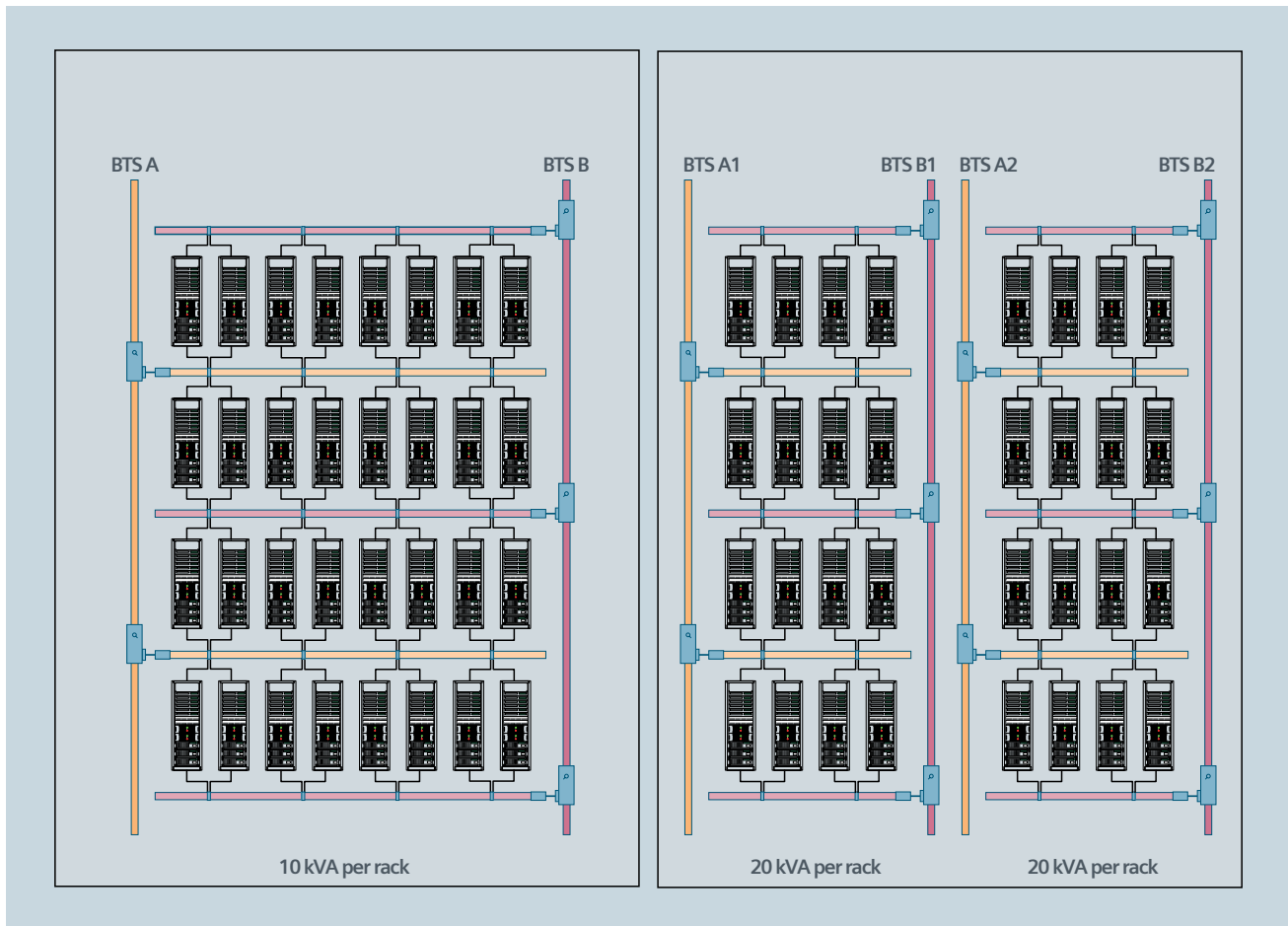
Fig. 2: Doubling of power with BTS in the server room
