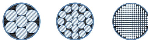
Figure 1 Class B stranded conductors, Class C stranded conductors, and fine stranded cable
