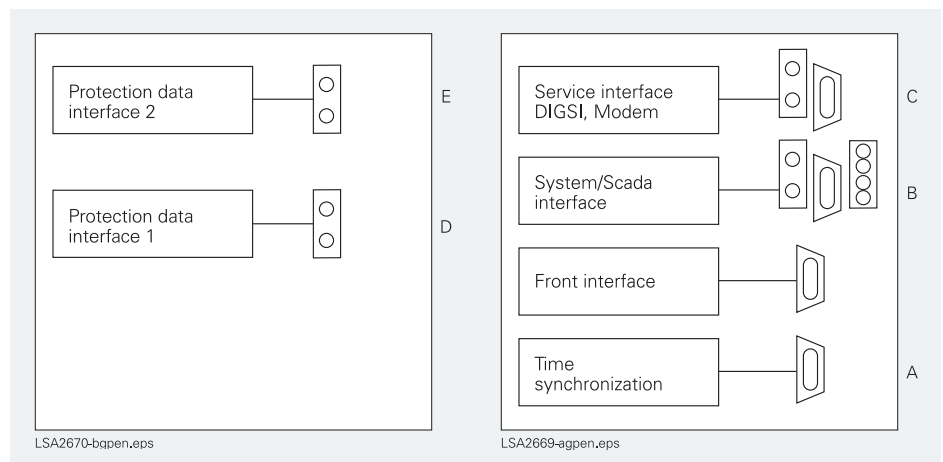
Fig. 7/74 Basic version in housing ½ x 19" with 8 binary inputs and 16 binary outputs
