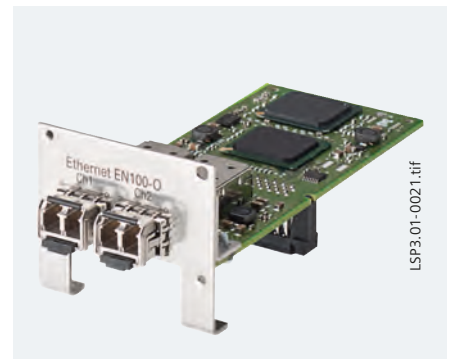
Fig. 7/54 Fiber-optic Ethernet communication module for IEC 61850 with integrated Ethernet switch
