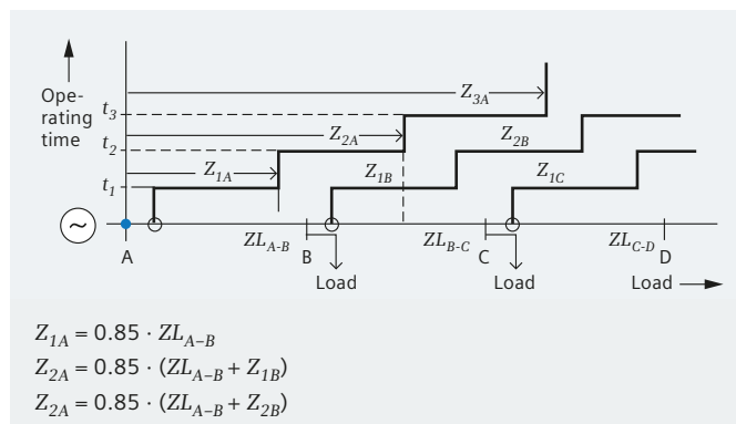
Fig. 2/84 Grading of distance zones
