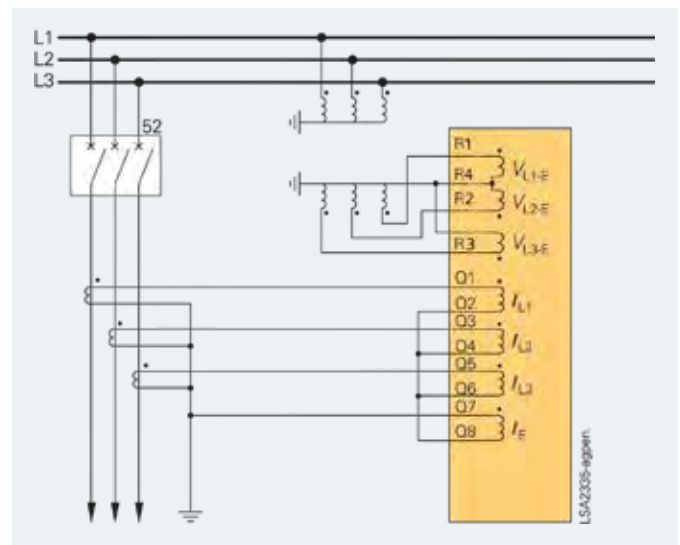
Fig. 5/106 Residual current circuit with directional element
