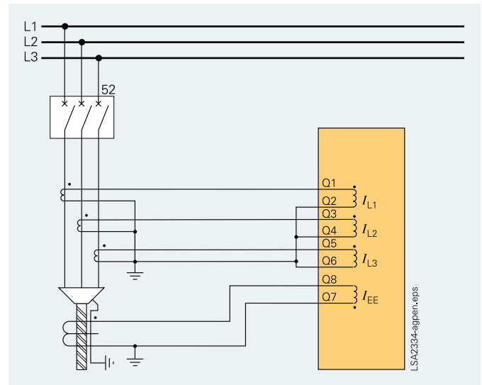
Fig. 5/105 Sensitive ground-current detection without directional element
