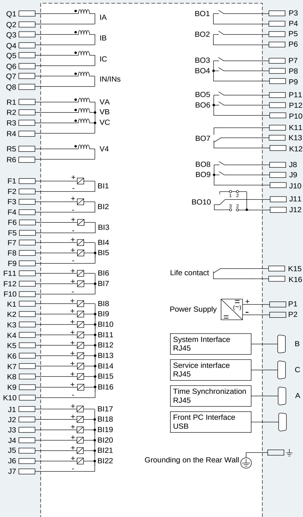
Fig. 5/115 SIPROTEC 7SJ662 connection diagram
