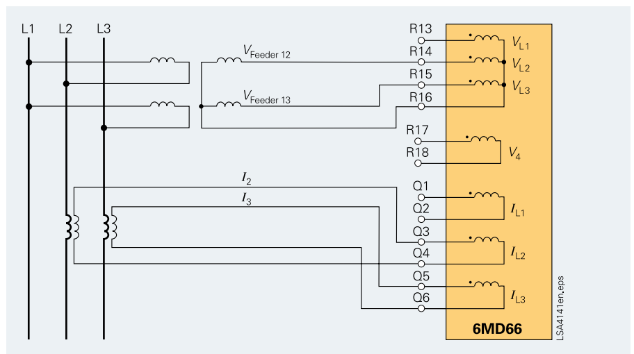
Fig. 12/17 Two-wattmeter circuit (connection to bay control unit)
