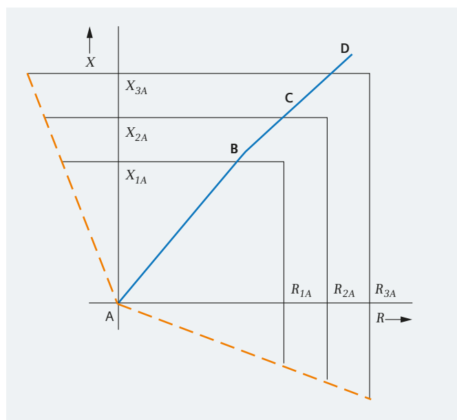
Fig. 2/85 Operating characteristics of Siemens distance relays
