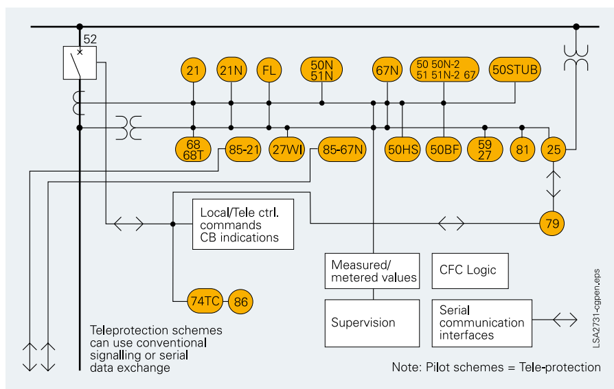
Fig. 6/47 Single-line diagram
