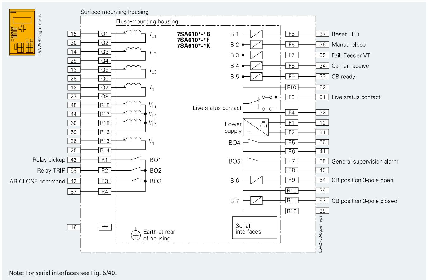
Fig. 6/40 Connection diagram
