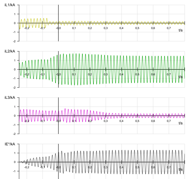
Figure 2: Phase and earth currents for single pole interruption
