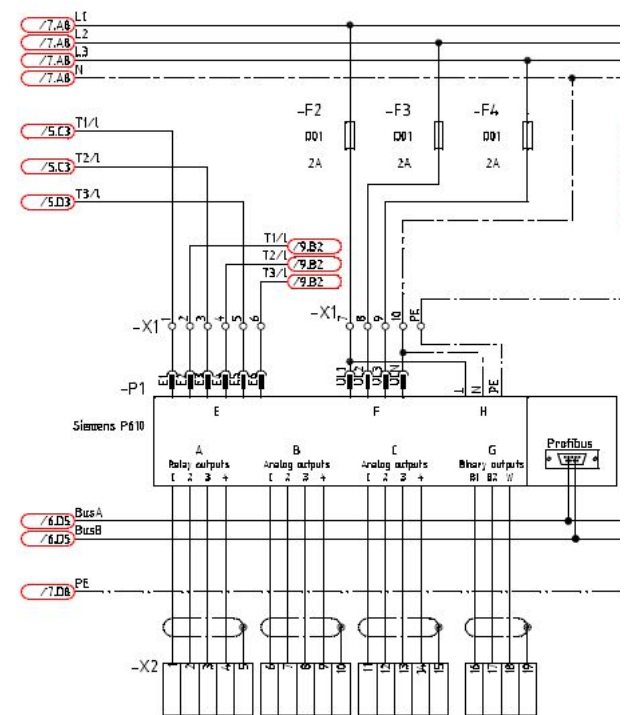
Figure 4: Secondary equipment configuration
