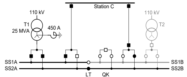
Figure 1: Substation configuration
