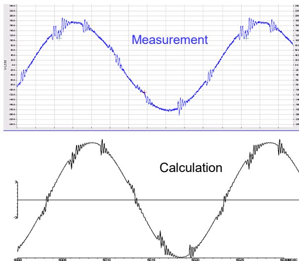
Figure 3: Simulated and measured voltage
