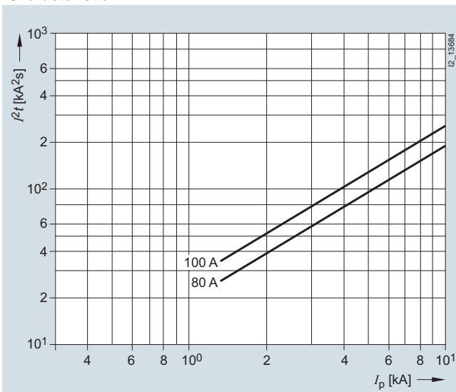
Characteristic D
