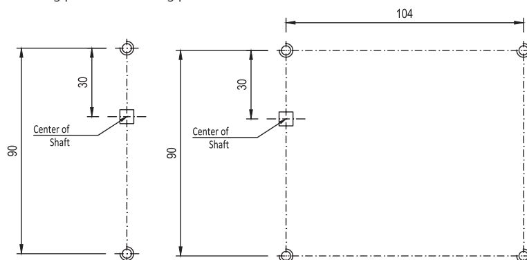
Drilling plan for mounting plate
