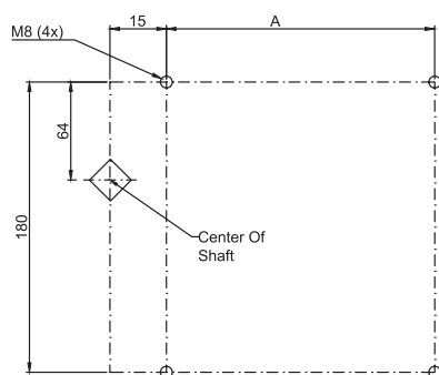
Drilling plan for mounting plate
