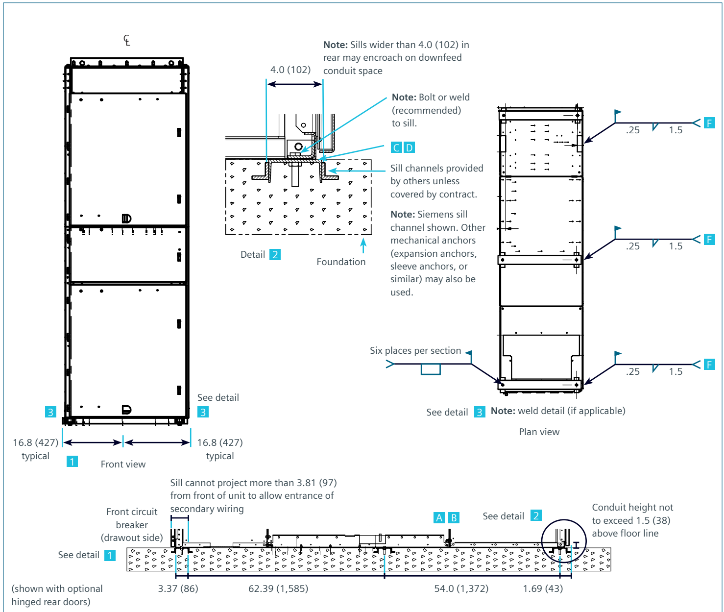
Figure 8b: (27kV): Anchoring indoor type GM-SG switchgear
