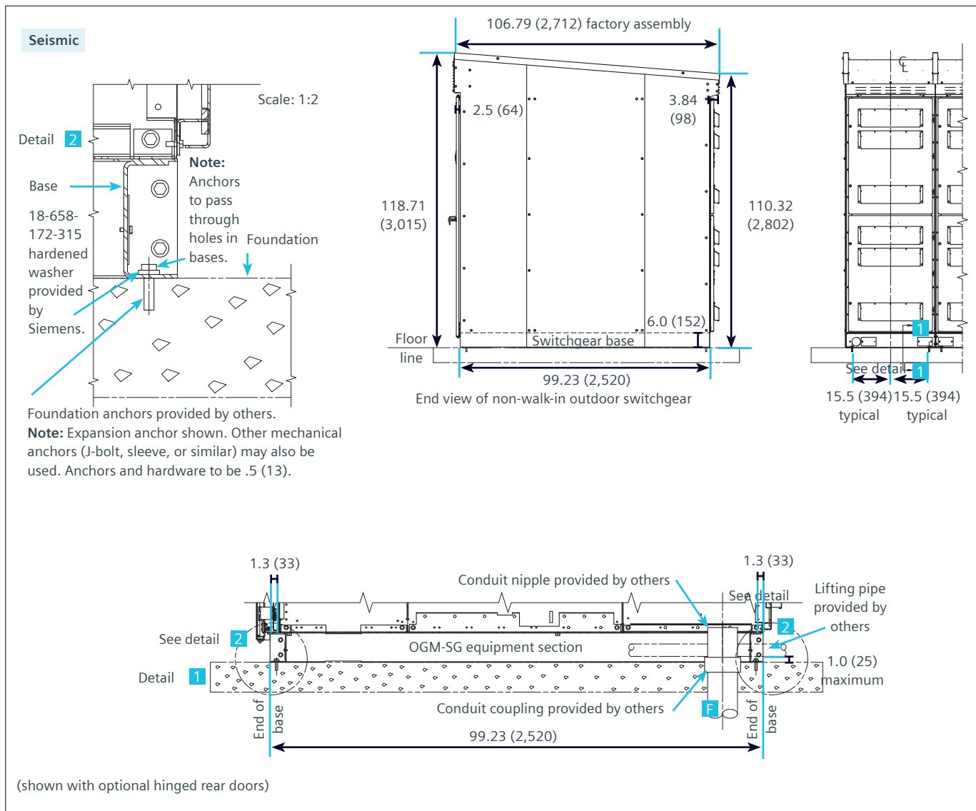
Figure 10a: (15 kV): Anchoring outdoor type OGM-SG non-walk-in switchgear
