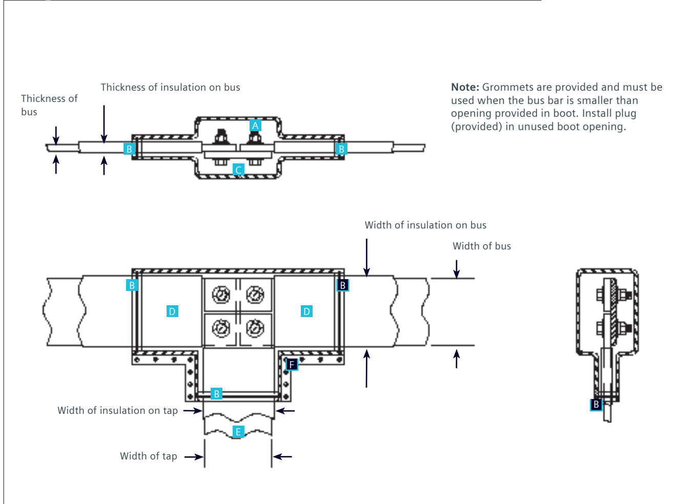
Figure 21: Typical installation of insulating boots
