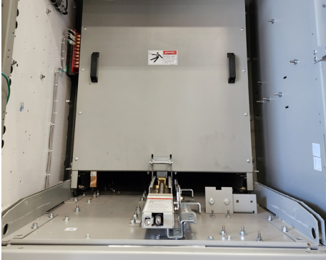
A. VT rollout tray in CONNECTED position. Handle/interlock bar fully extended to secure VT rollout tray in cell.
