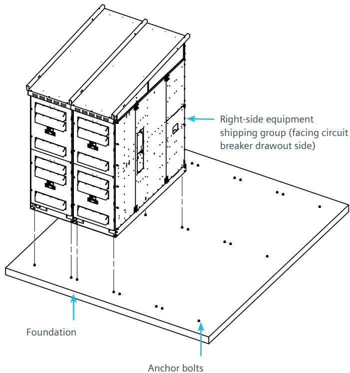
Figure 3: Right-side shipping group installed
