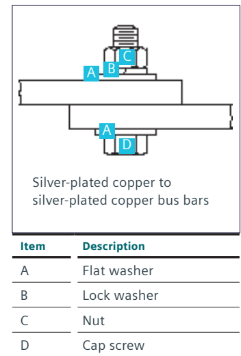
Figure 19: Main bar joint assembly
