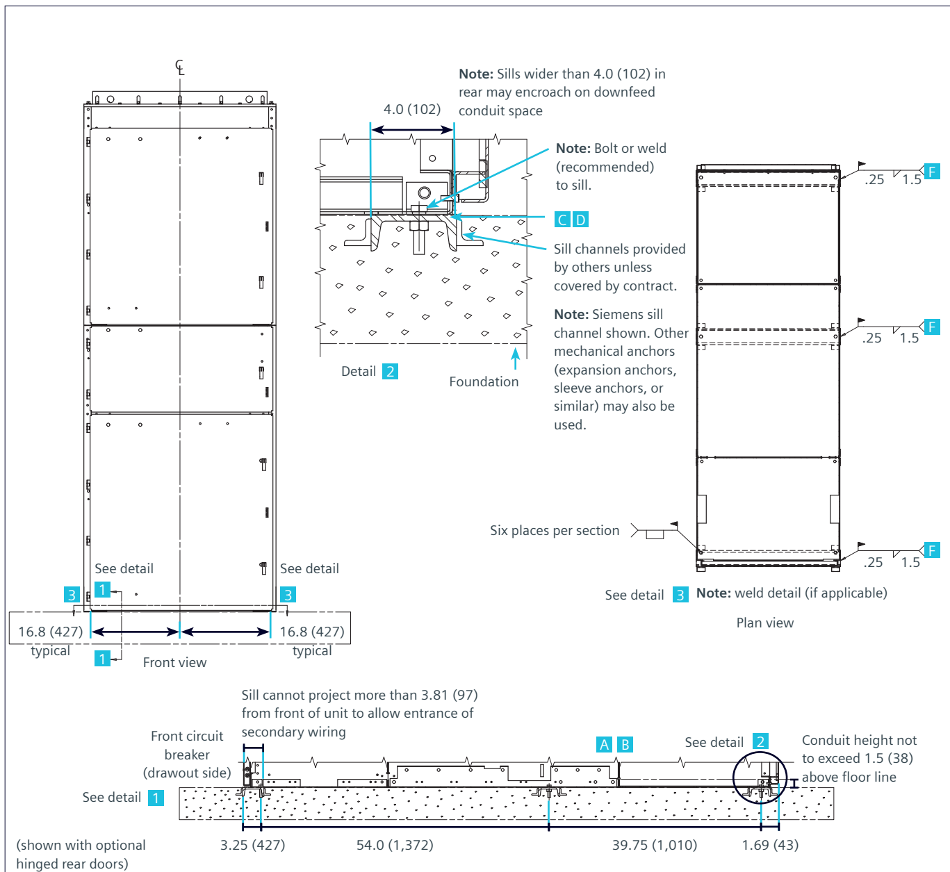
Figure 8a: (15 kV): Anchoring indoor type GM-SG switchgear
