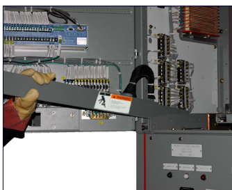
Figure 40: Use of extension rails for removal of circuit breaker from upper compartment
