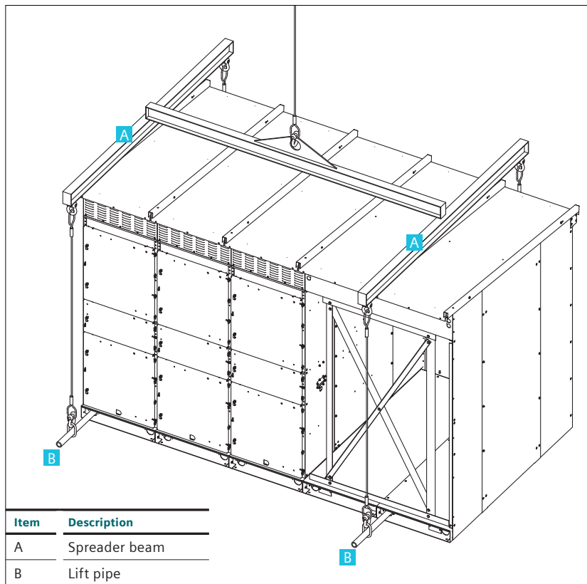
Figure 5: Lifting outdoor switchgear with crane
