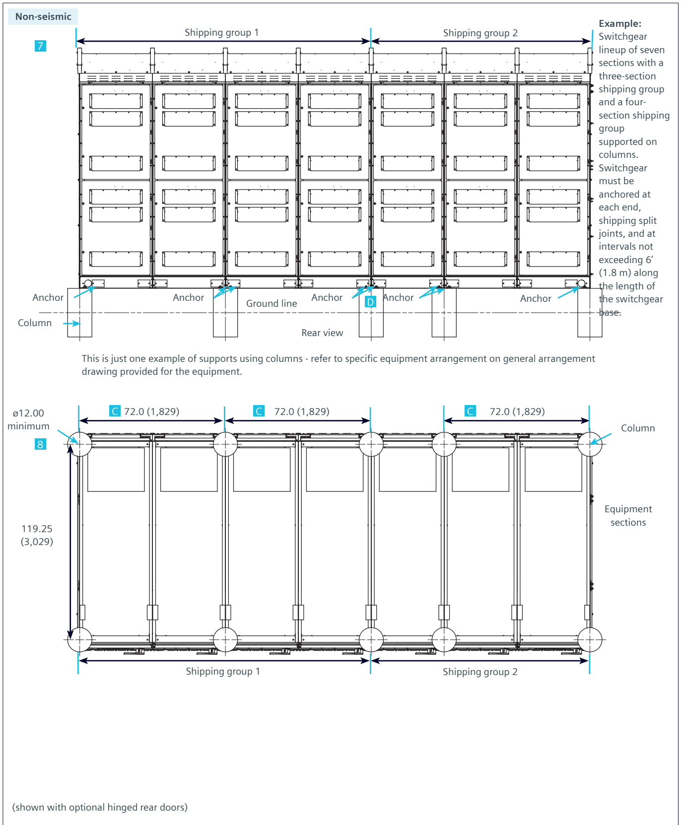
Figure 10b: (27 kV): Anchoring outdoor type OGM-SG non-walk-in switchgear (continued)
