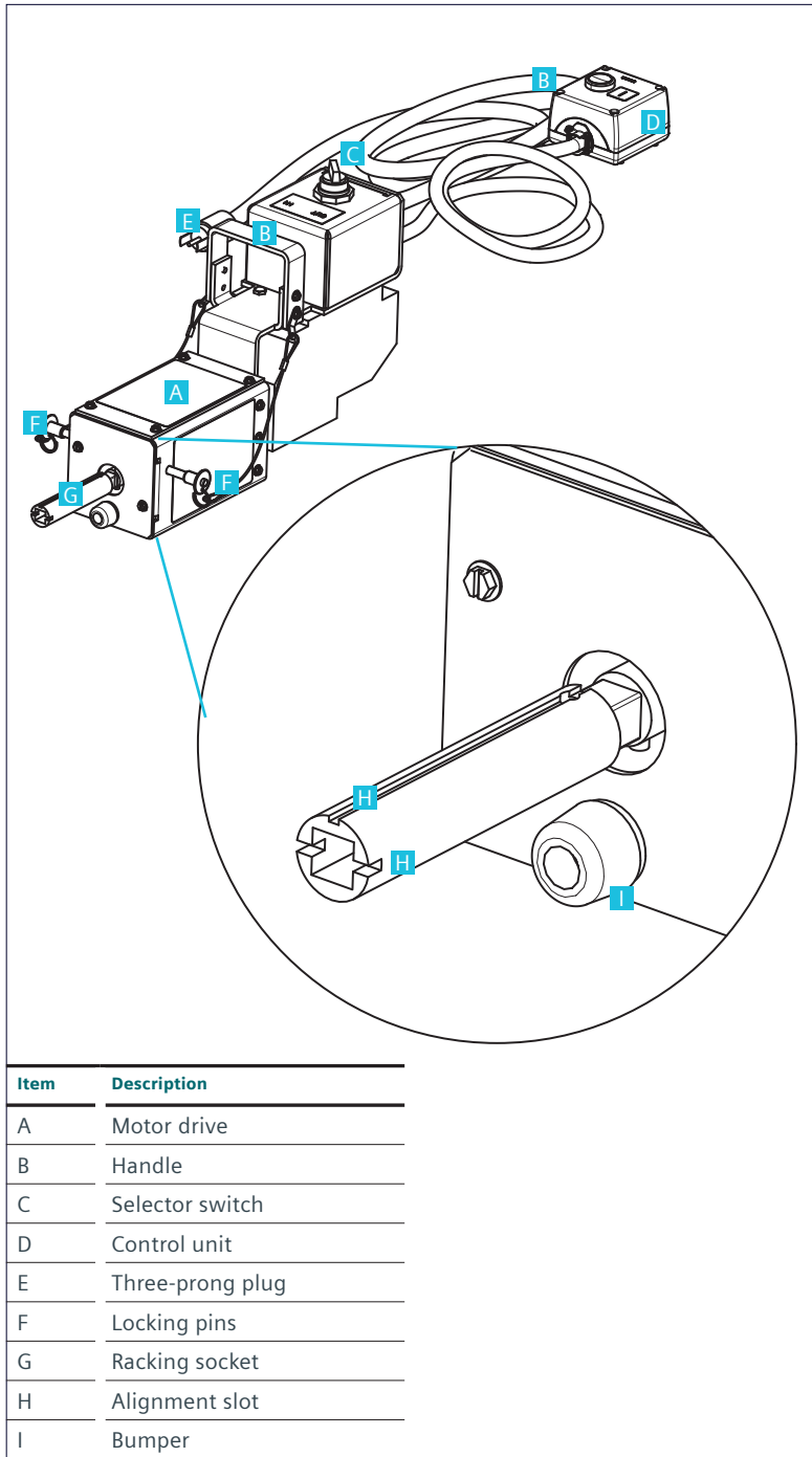
Figure 57: Electrical-racking device
