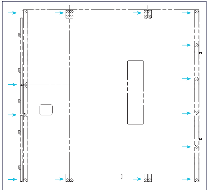
Figure 12: Interunit bolting location
