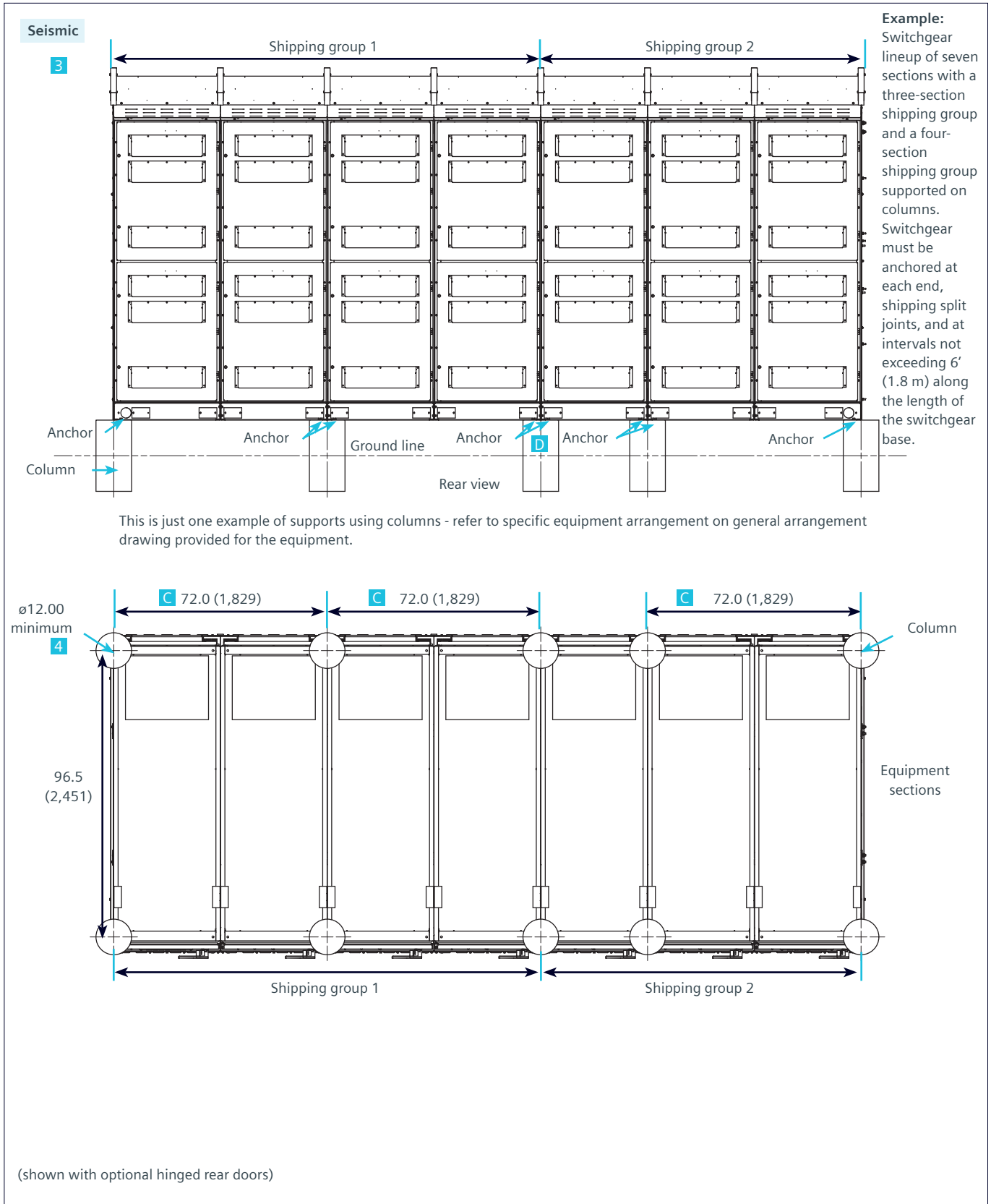
Figure 10a: (15 kV): Anchoring outdoor type OGM-SG non-walk-in switchgear (continued)
