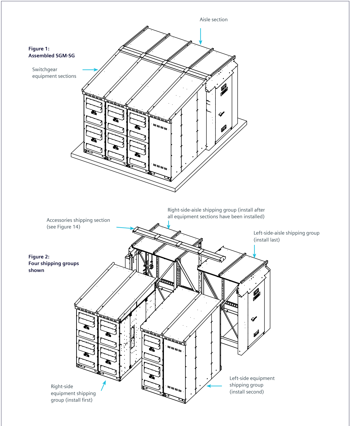
Figure 13: Instructions for factory-assembled-aisle type SGM-SG
