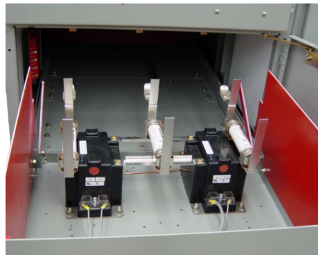
D. VT rollout tray withdrawn to allow inspection of fuses.
