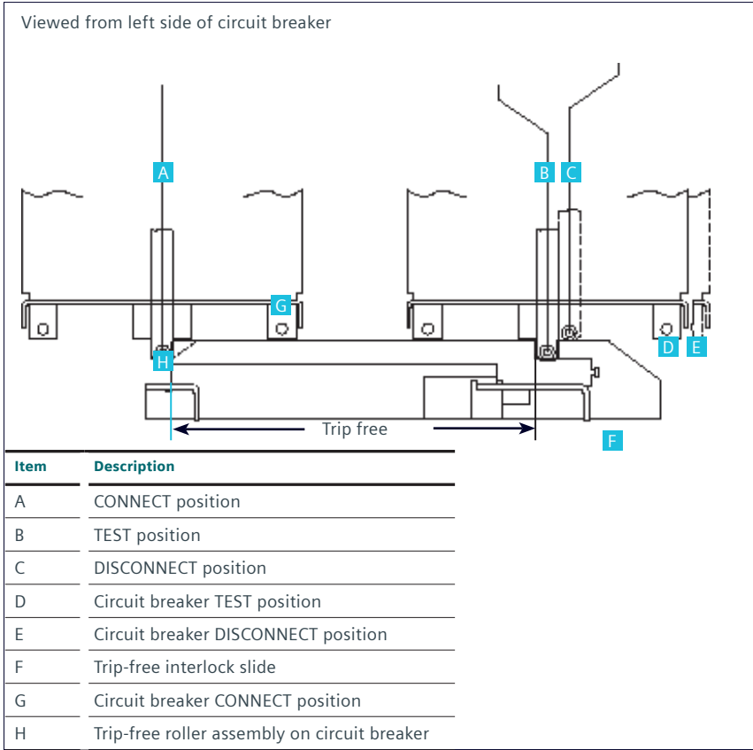
Figure 46: Trip-free interlock arrangement
