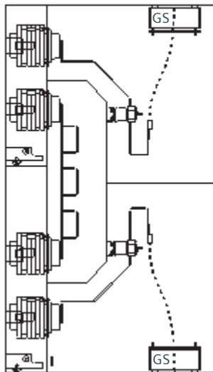
C. Two circuit breakers. Upper cables top exit. Lower cables bottom exit.
