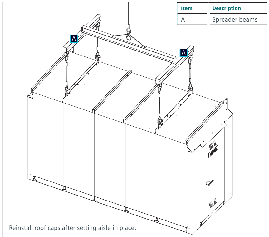
Figure 6: Moving the aisle portion of outdoor switchgear
