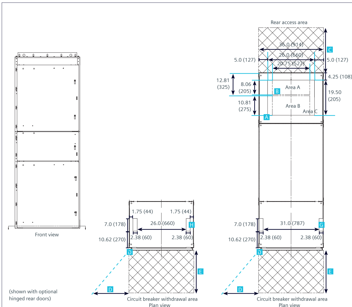
Figure 8a: (15 kV): Anchoring indoor type GM-SG switchgear (continued)
