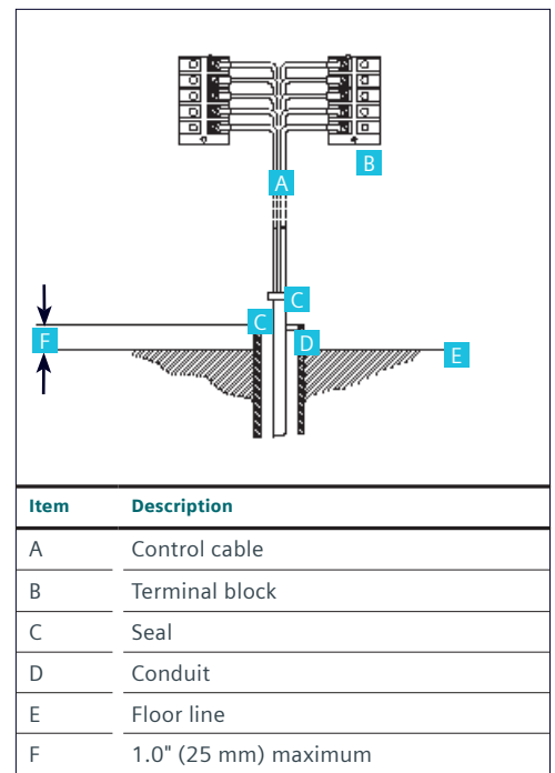
Figure 27: Secondary control cable connections
