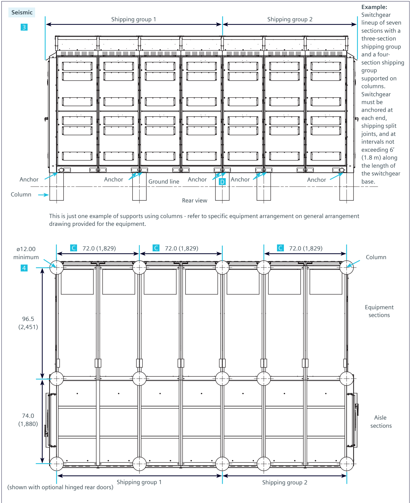
Figure 9a: (5-17.5kV) Anchoring outdoor type SGM-SG Shelter-Clad single-aisle switchgear (continued)
