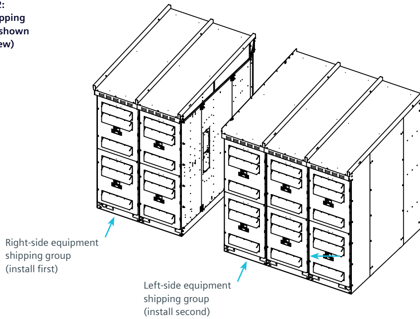
Figure 15: Instructions for non-walk-in type OGM-SG switchgear
