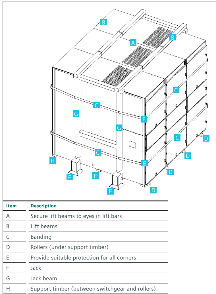
Figure 3: Moving switchgear with jacks and rollers
