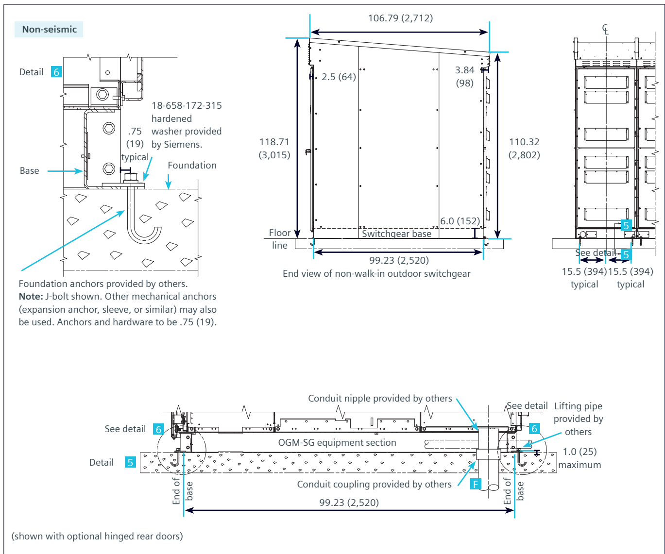
Figure 10a: (15 kV): Anchoring outdoor type OGM-SG non-walk-in switchgear (continued)
