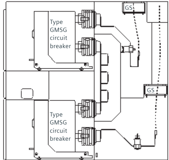
B. Two feeder circuit breakers. Cables top exit.
