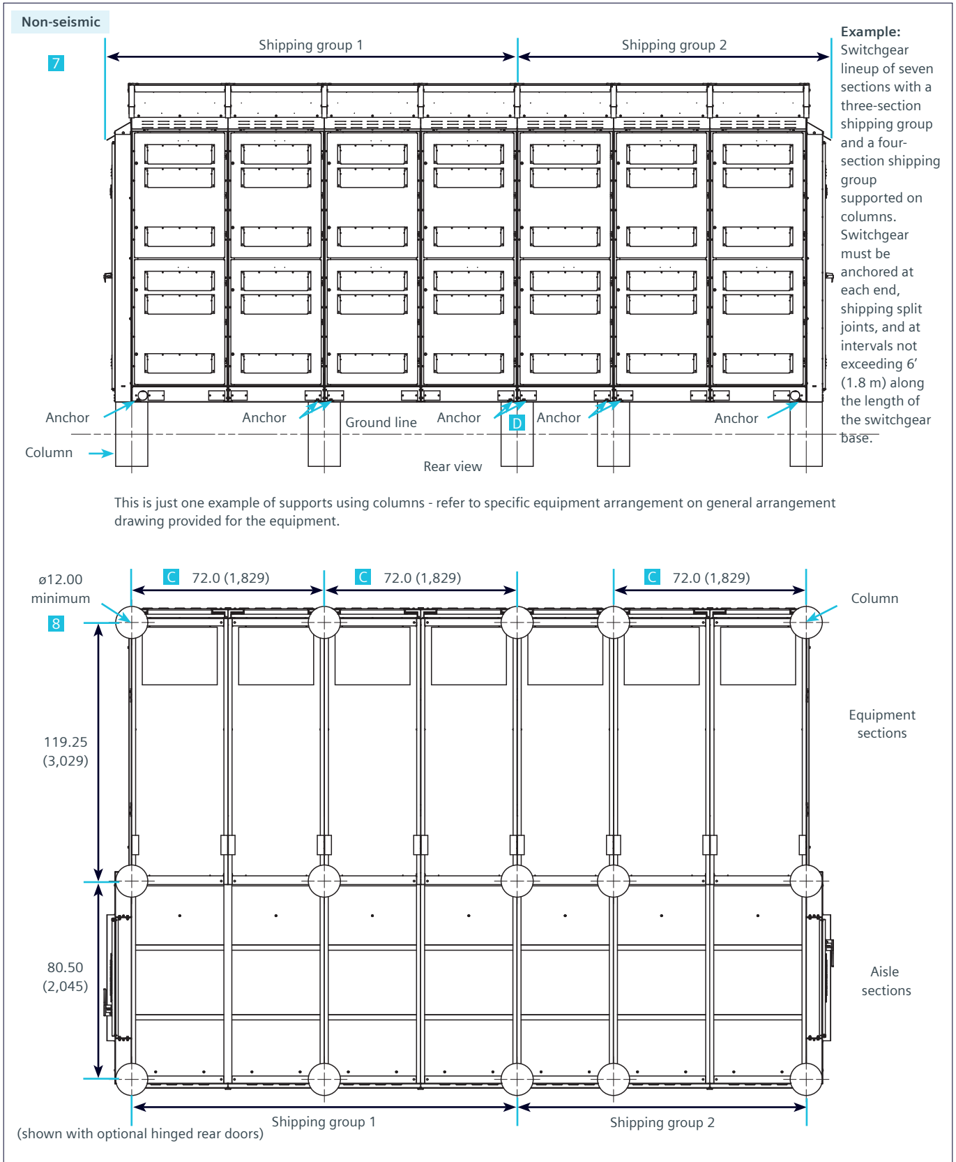
Figure 9b: (27kV) Anchoring outdoor type SGM-SG Shelter-Clad single-aisle switchgear (continued)
