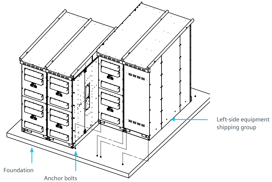
Figure 5: Left-side shipping group installed
