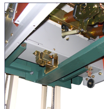
Figure 51: Front support locations
