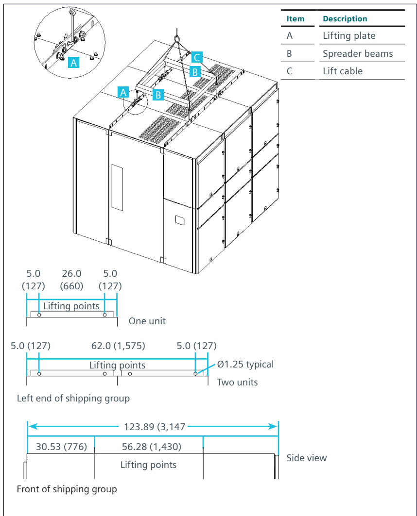
Figure 2b: Lifting indoor switchgear with crane (27 kV only)
