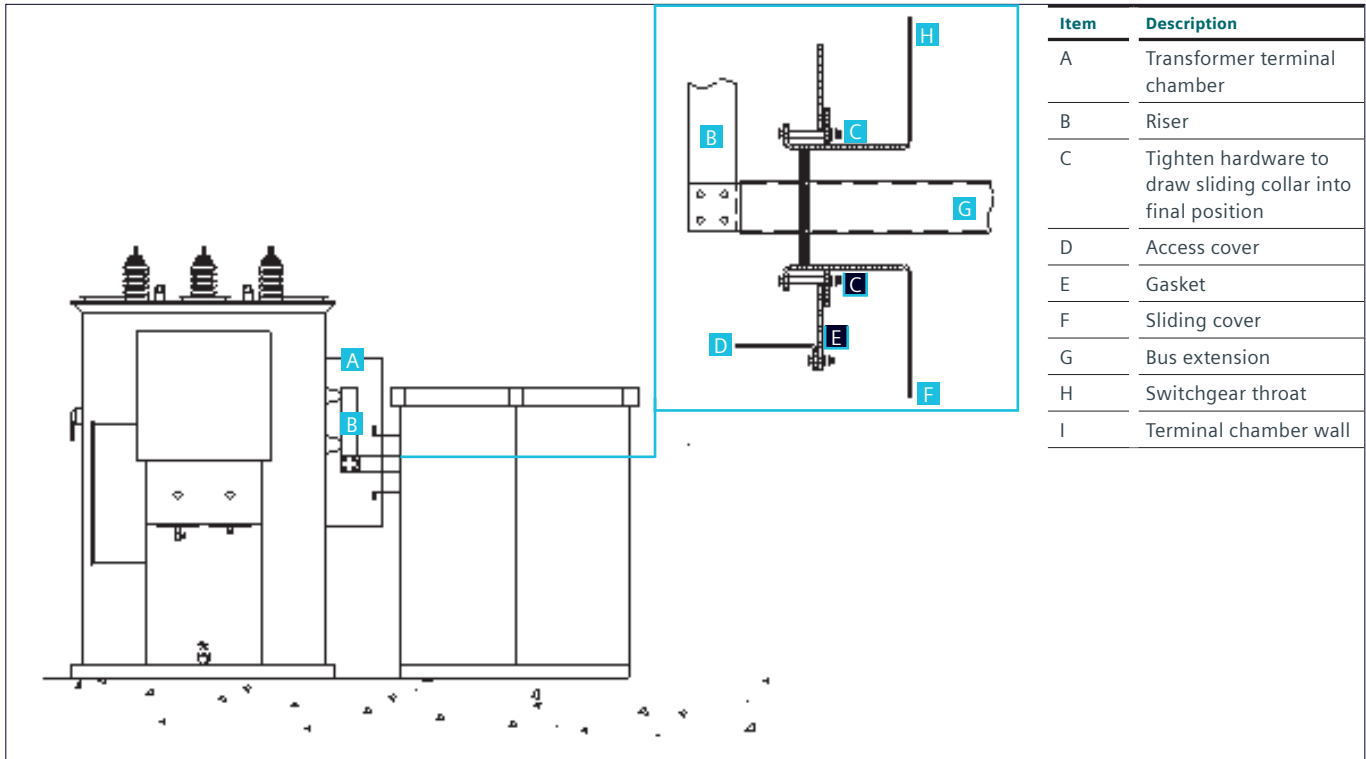
Figure 11: Throat connection
