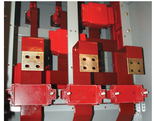
Figure 26: Typical cable termination compartment (bus compartment covers removed)
