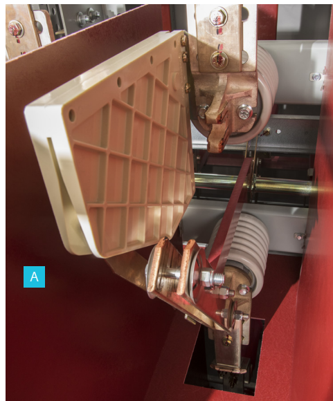
Figure 67: Checking proper alignment
