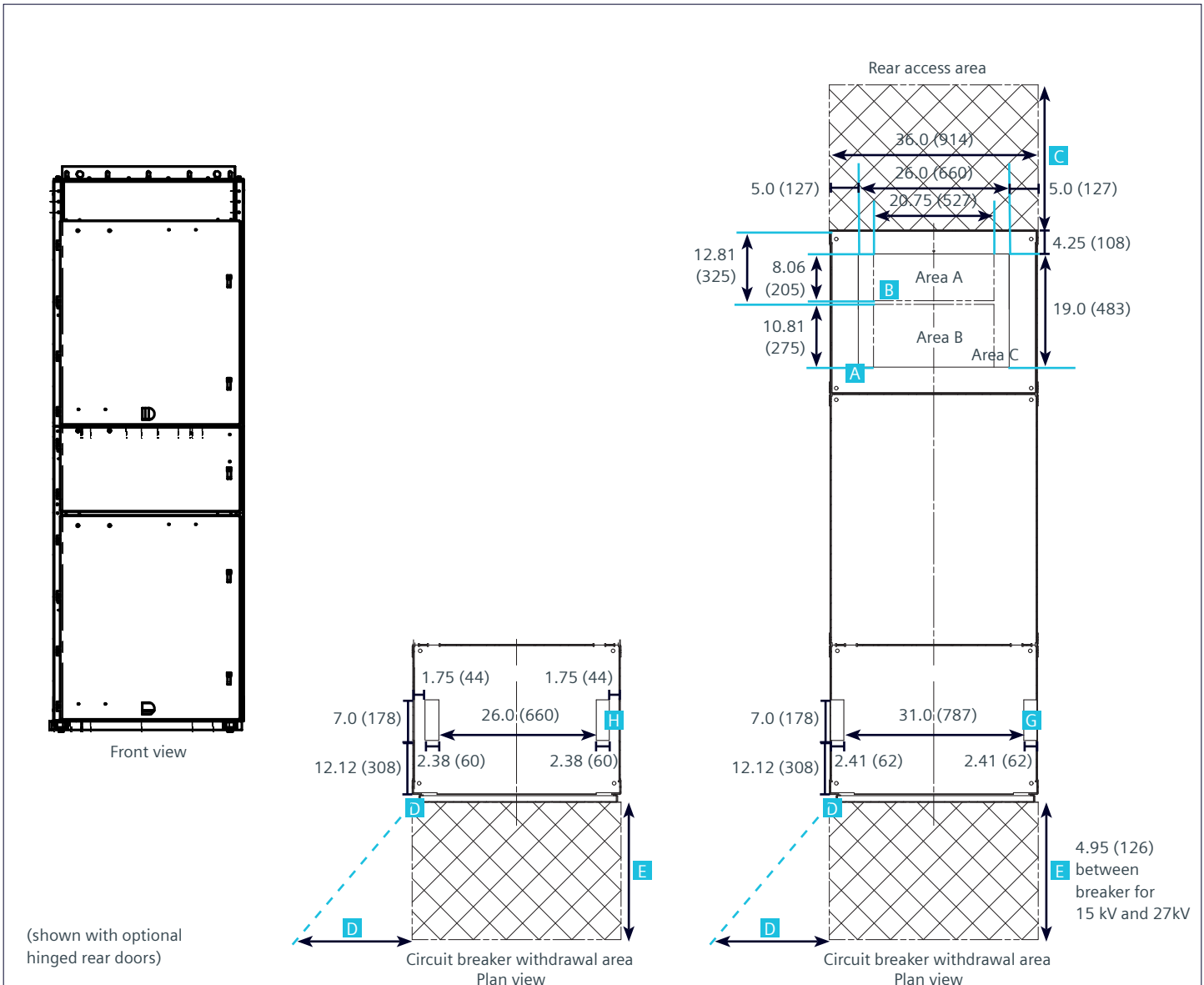
Figure 8b: (27 kV): Anchoring indoor type GM-SG switchgear (continued)
