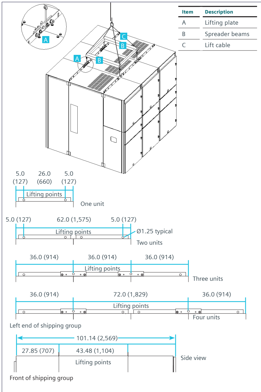
Figure 2a: Lifting indoor switchgear with crane
