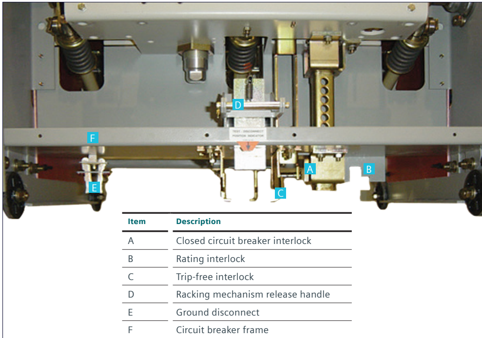
Figure 35: Interlocks on bottom of circuit breaker
