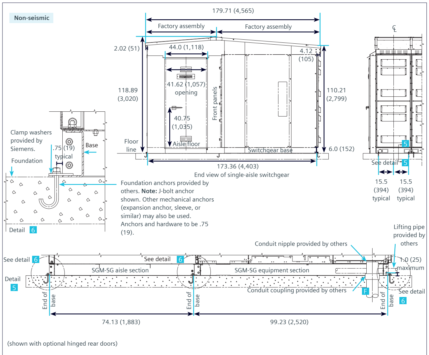
Figure 9a: Figure 9a: (5-17.5kV) Anchoring outdoor type SGM-SG Shelter-Clad single-aisle switchgear (continued)
