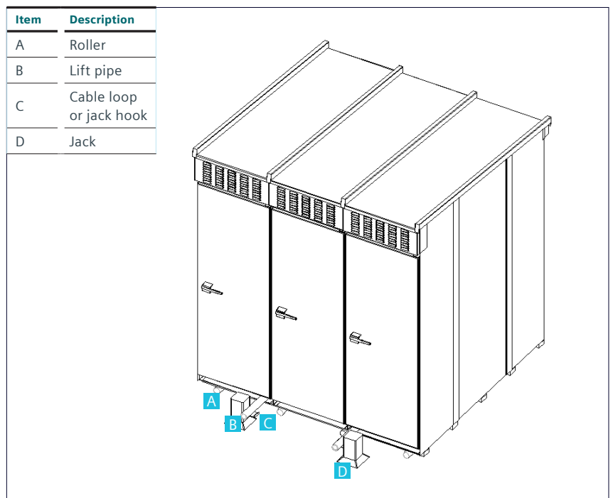
Figure 7: Moving outdoor switchgear with jacks and rollers
