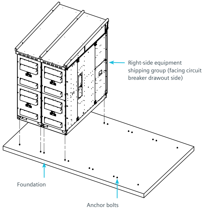
Figure 3: Right-side shipping group installed
