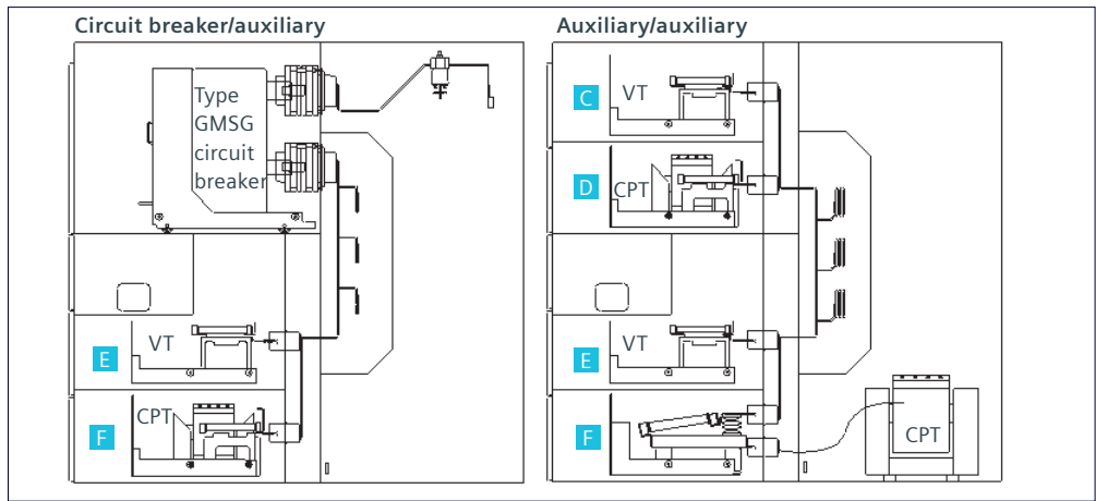
Figure 30a: Typical VT, CPT and CPT fuse rollout configuration
