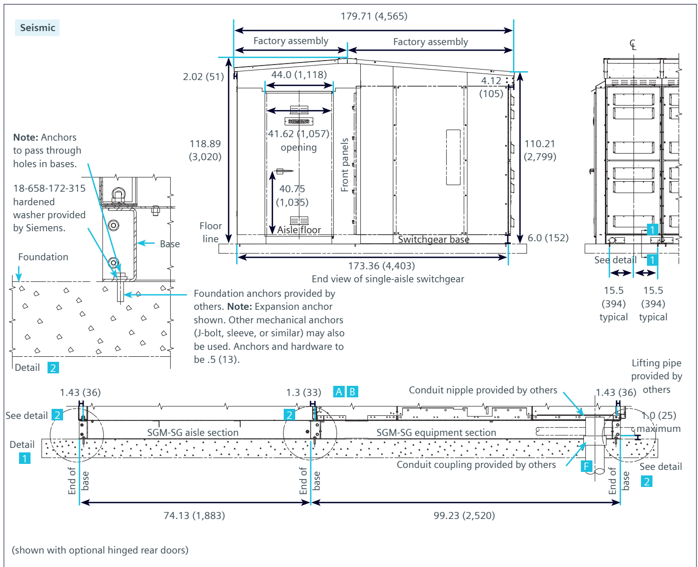
Figure 9a: (5-17.5kV) Anchoring outdoor type SGM-SG Shelter-Clad single-aisle switchgear
