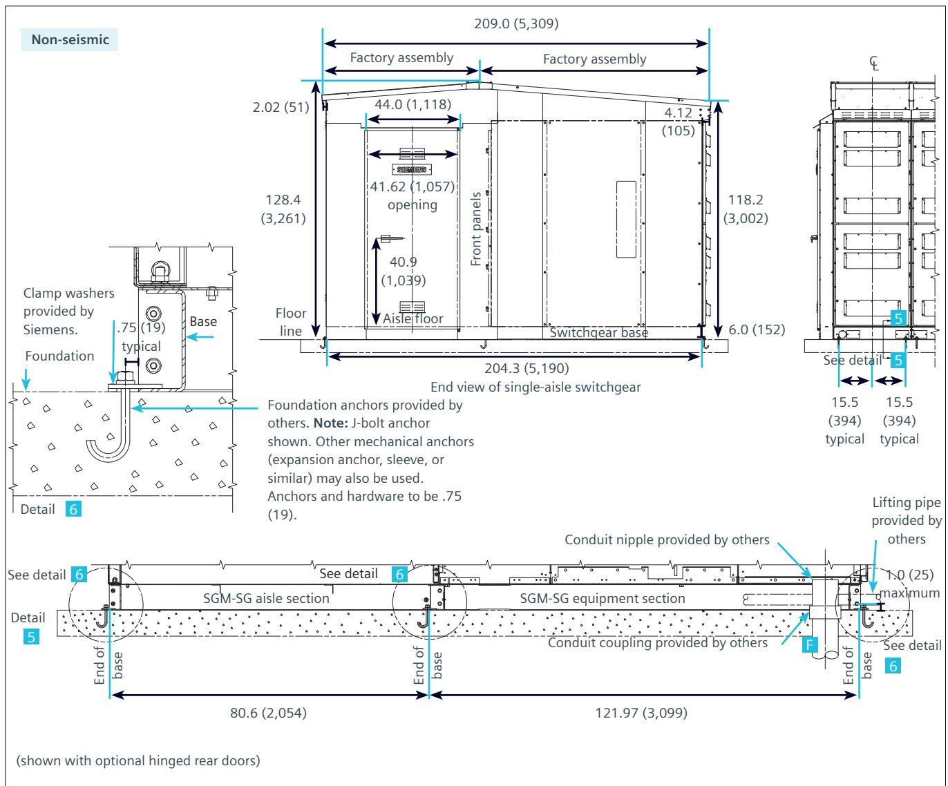
Figure 9b: (27kV) Anchoring outdoor type SGM-SG Shelter-Clad single-aisle switchgear (continued)
