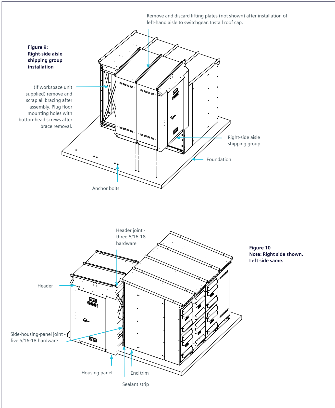
Figure 13: Instructions for factory-assembled-aisle type SGM-SG (continued)
