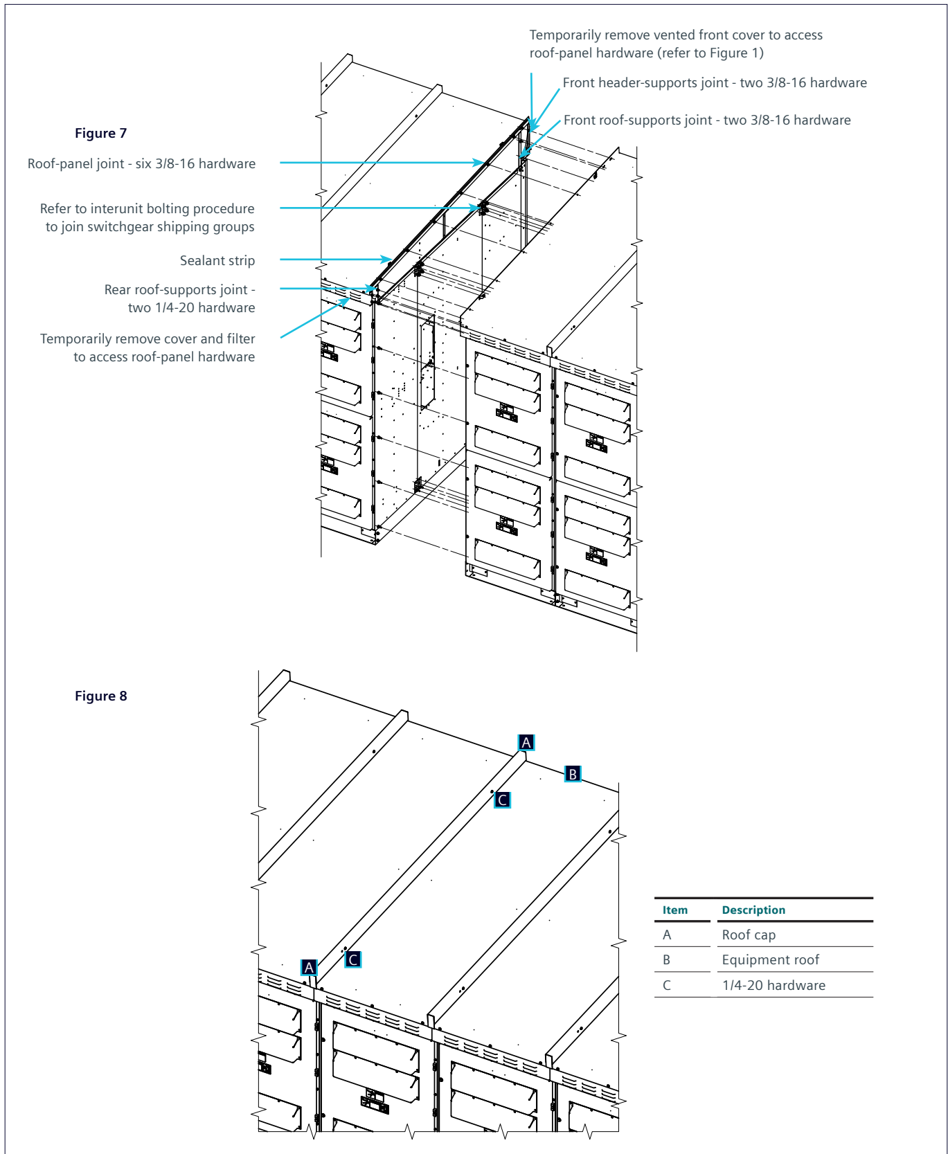
Figure 15: Instructions for non-walk-in type OGM-SG switchgear (continued)
