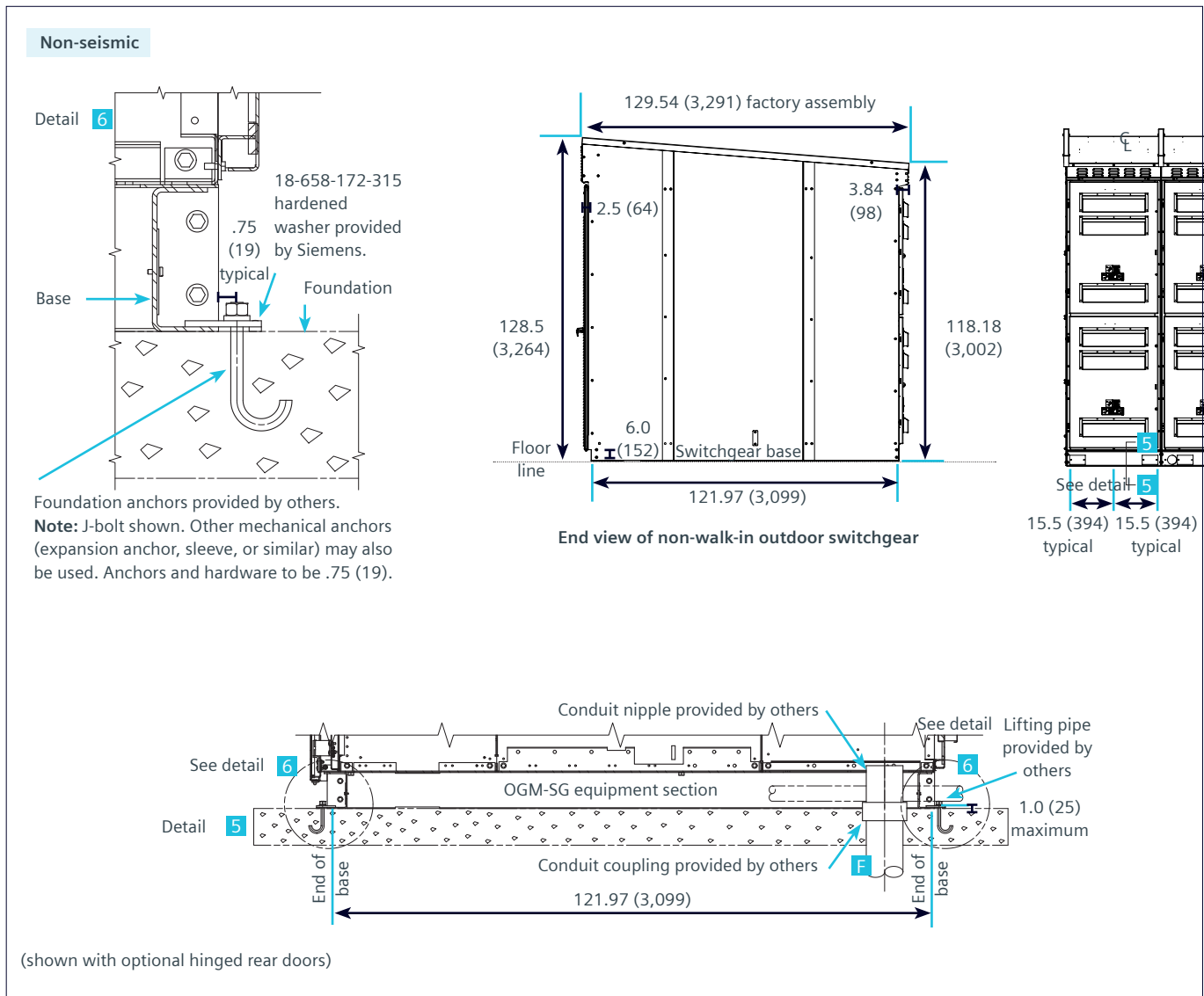
Figure 10b: (27 kV): Anchoring outdoor type OGM-SG non-walk-in switchgear (continued)
