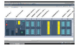
TIA PORTAL DEVICE VIEW
