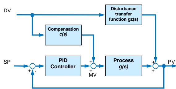
Figure 7: Feedforward disturbance compensation, DV: Disturbance Variable
