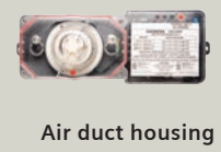
Air duct housing with relays FDBZ492-HR Order no.: S54319-B23-A1
