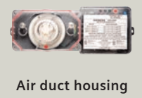
Air duct housing FDBZ492 Order no.: S54319-B22-A1
