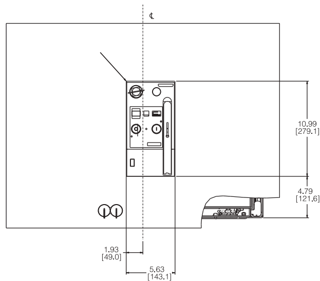
Minimal door cut-out (Only center eustcheon visible)
