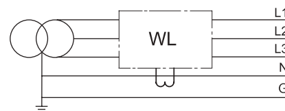
Residual sensing of the ground fault current
