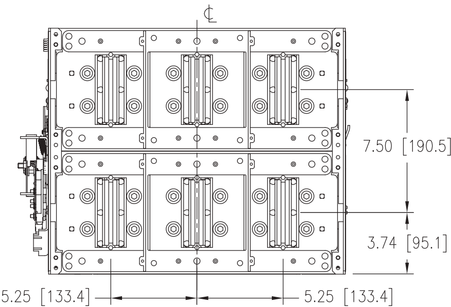
Rear view
