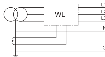
Direct measurement of the ground fault current
