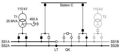
Figure 1: Substation configuration
