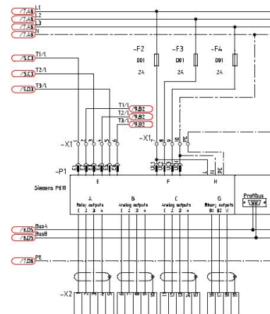
Figure 4: Secondary equipment configuration
