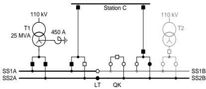
Figure 1: Substation configuration
