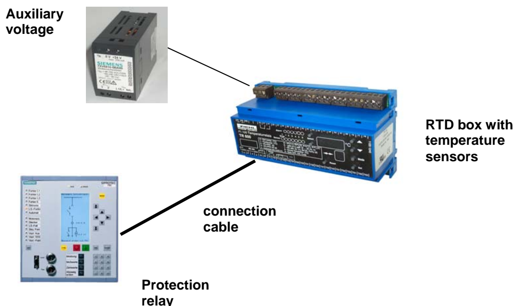
Picture 1: Overview for the application of RTD box
