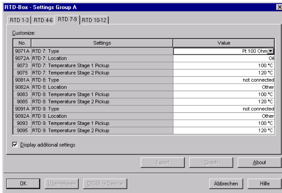
Picture 13: Setting of parameters
