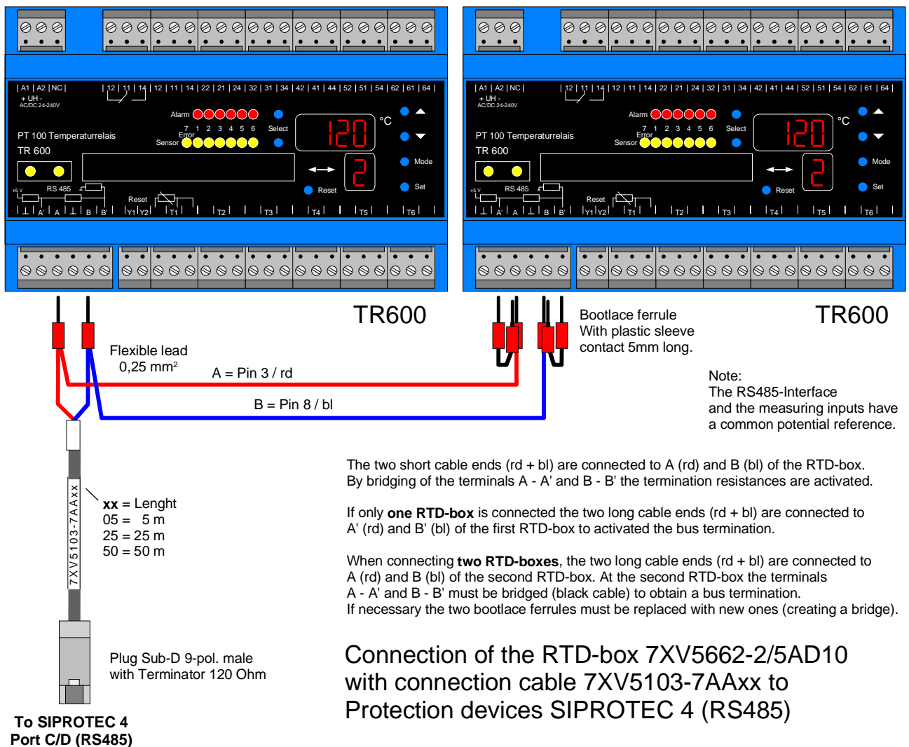
Picture 5: Connection RTD-box to SIPROTEC 4
