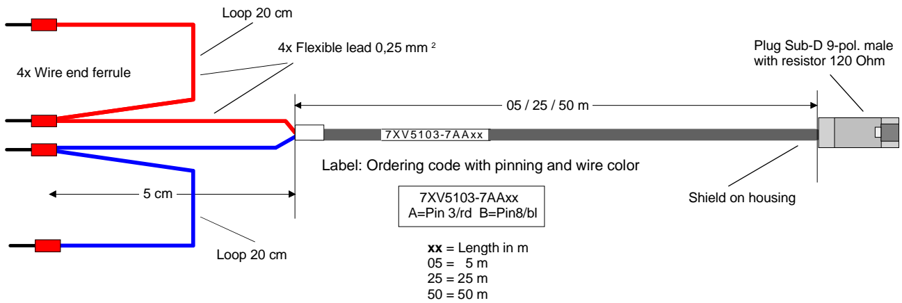
Picture 4: Cable 7XV5103-7xx for RS485-bus with 9-pol. Sub-D plug
