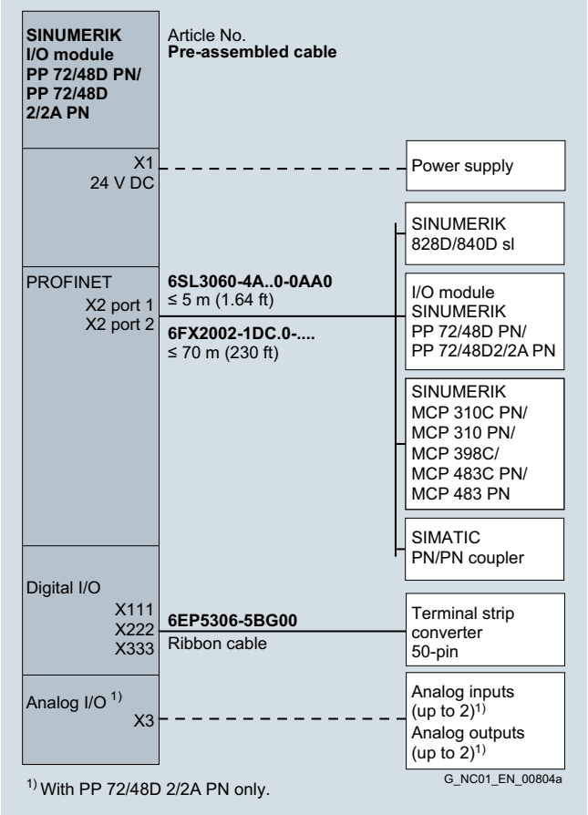
Connection overview of SINUMERIK PP 72/48D PN and PP 72/48D 2/2A PN I/O modules
