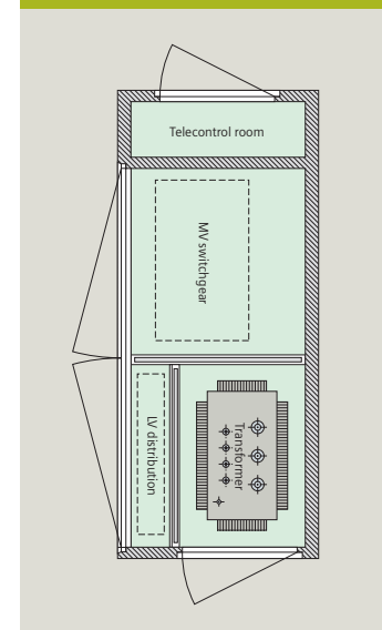
Typical room planning of a transformer substation
