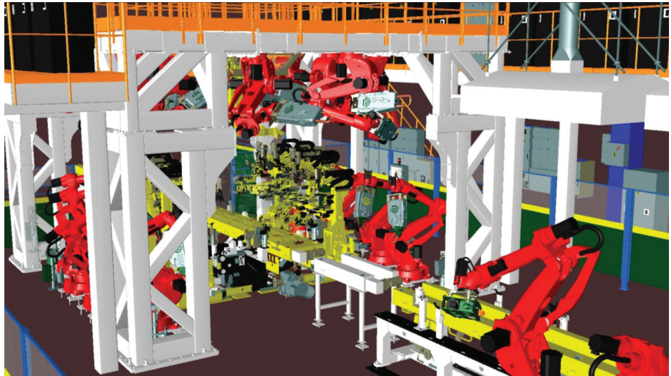
A physical, commissioned welding station delivered to Fiat, and the virtual workcell simulated using Tecnomatix.
