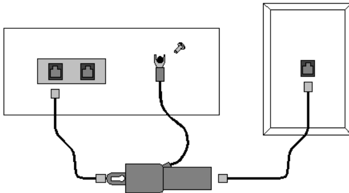
Figure 1. Typical Telephone or Fax Installation
