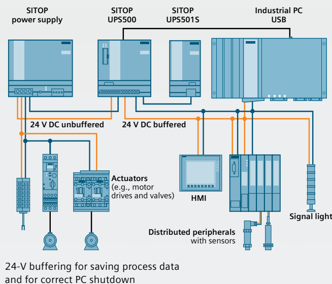
SITOP DC UPS configuration with capacitors
