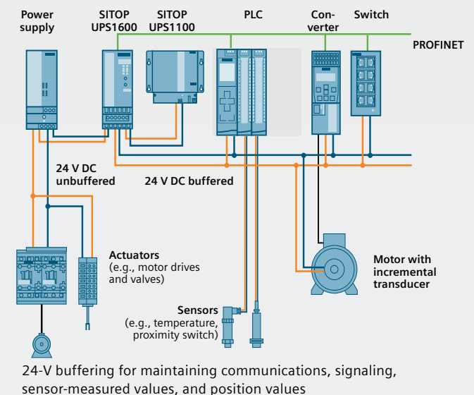
SITOP DC UPS configuration with battery modules
