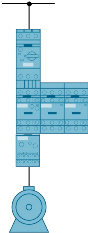
Setup of a motor feeder with contactor assembly for star-delta start
