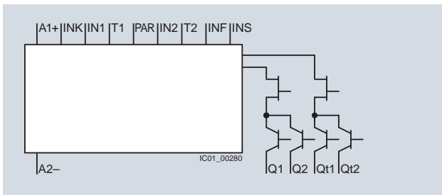
3SK1122-.CB4, Advanced solid-state instantaneous basic unit
