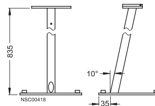
3SU1950-0HN10-0AA0 stand
