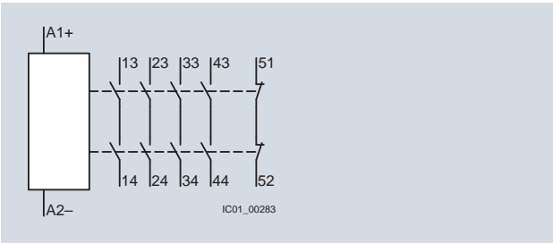
4RO 3SK1211 output expansion
