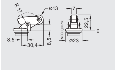
Angular roller lever
