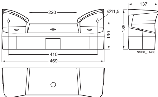
3SU1853-3NB00-1AA1 operator panel with metal enclosure
