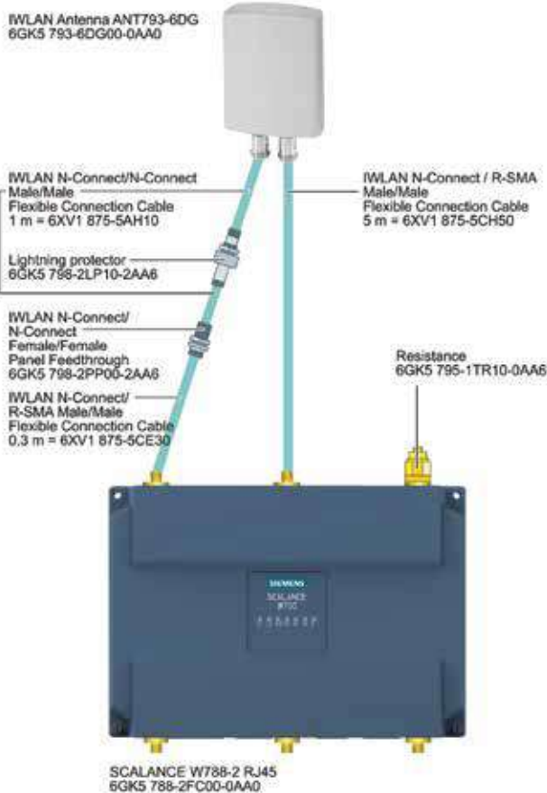
Dual Slant antenna ANT793-6DG connected to SCALANCE W788-2 RJ45 with R-SMA parts
