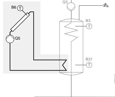
DHW charging collector pump, collector sensor
