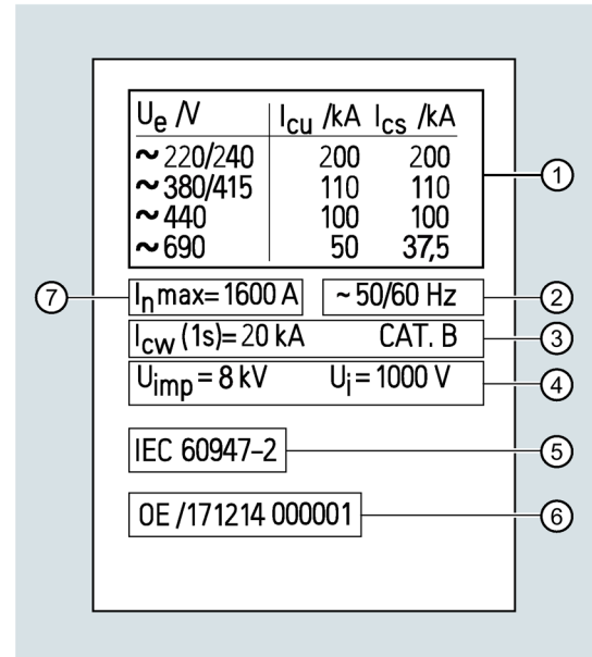
Circuit breaker
