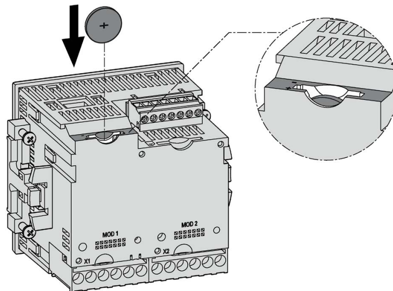
Figure 8-3 Battery change
