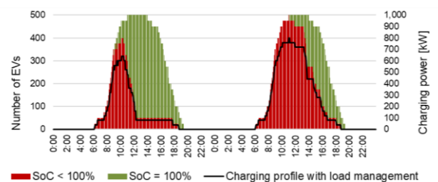
Figure 2: Exemplary results of a charging profile simulation
