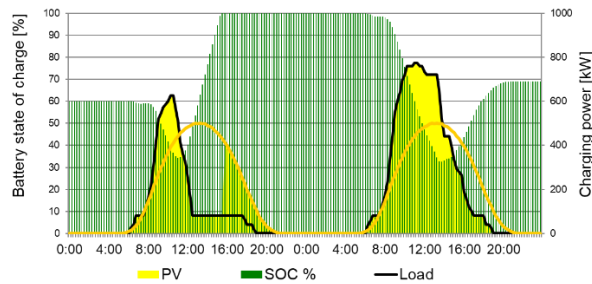
Figure 3: Exemplary simulation of PV and energy storage to cover the load demand
