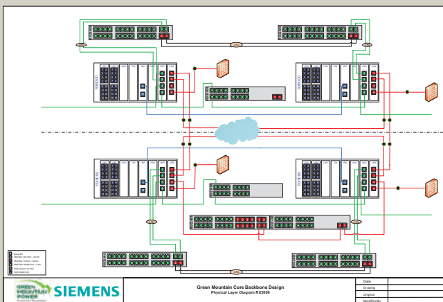
Green Mountain Power Core Backbone Design
