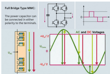
Figure 1: Basic HVDC Plus concept
