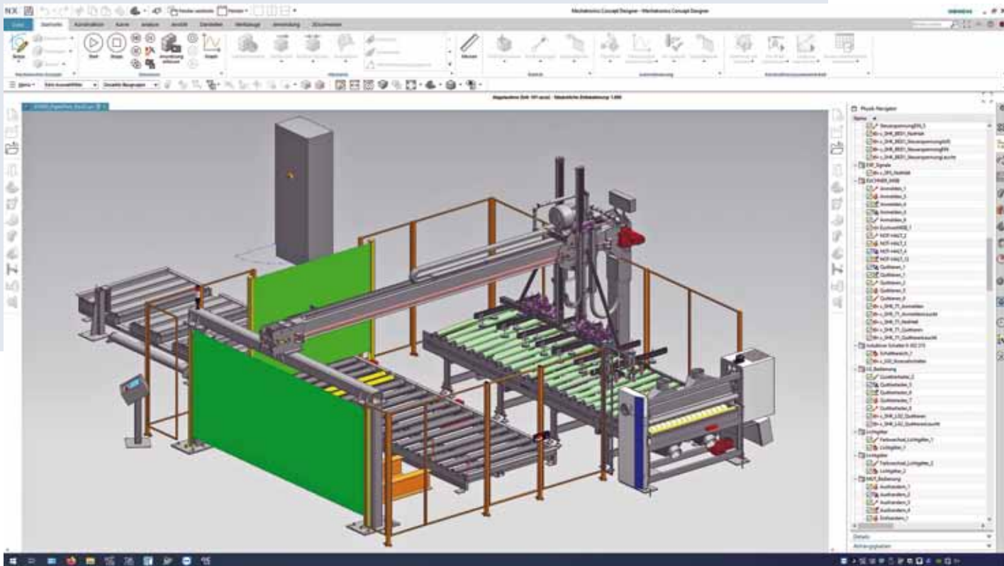
Screen view of a CAD drawing for the gantry feeder with protection board storage (see also original photo of the system for comparison). Full view without overlays
