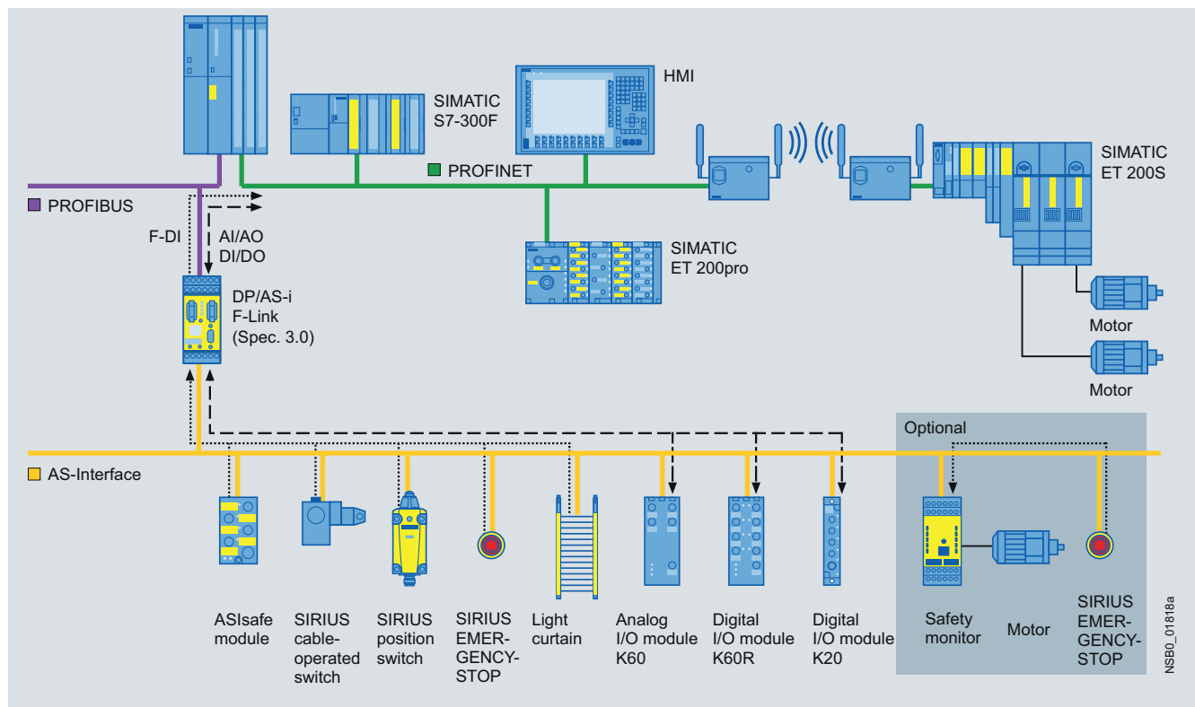
Integration in PROFINET networks under SIMATIC F-SPS (alternatively can also be integrated through IE/PB Link)
